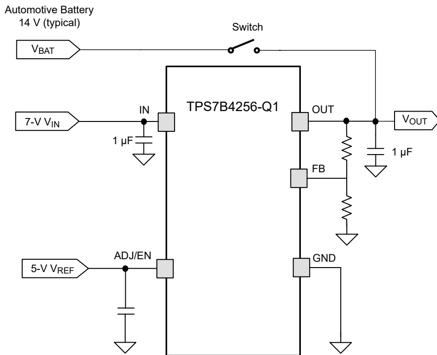
☒ 6-7. Output Voltage Higher Than the Input
