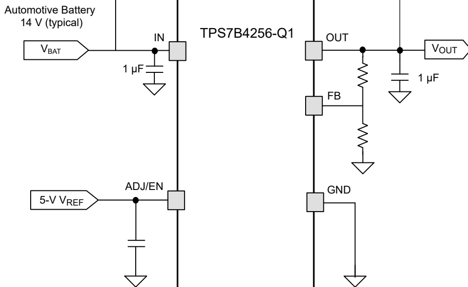
☒ 6-6. Output Voltage Short to Battery
