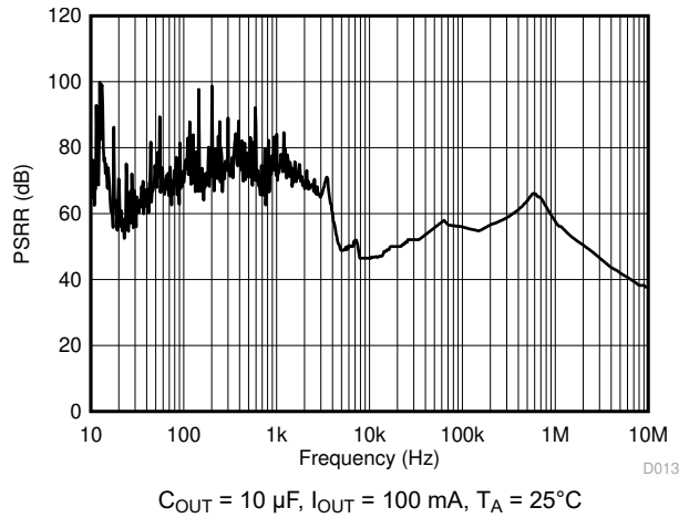
图 5-13. PSRR vs Frequency
