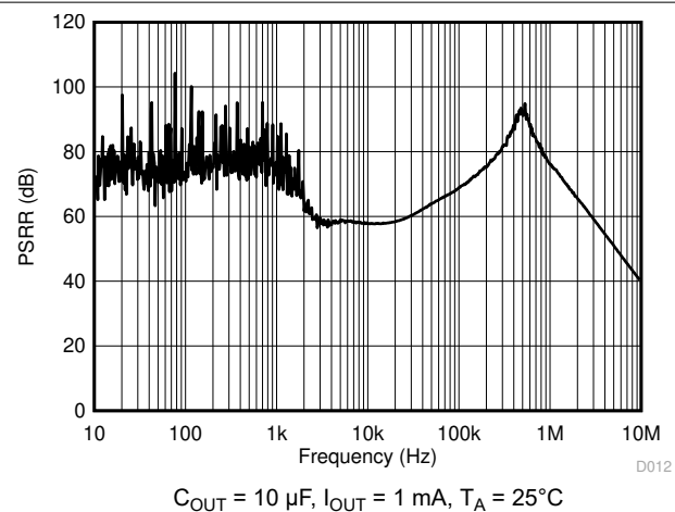
図 5-12. PSRR vs Frequency
