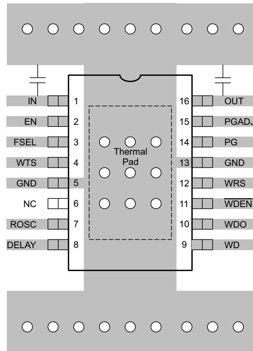
7-4. Layout Recommendation
