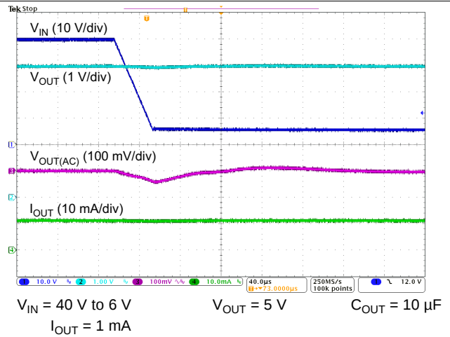
FIG 16. Line Transient
