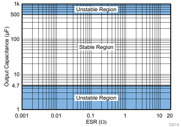
FIG 14. ESR Stability vs Output Capacitance
