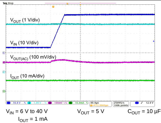
FIG 15. Line Transient
