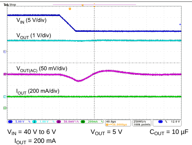
FIG 18. Line Transient
