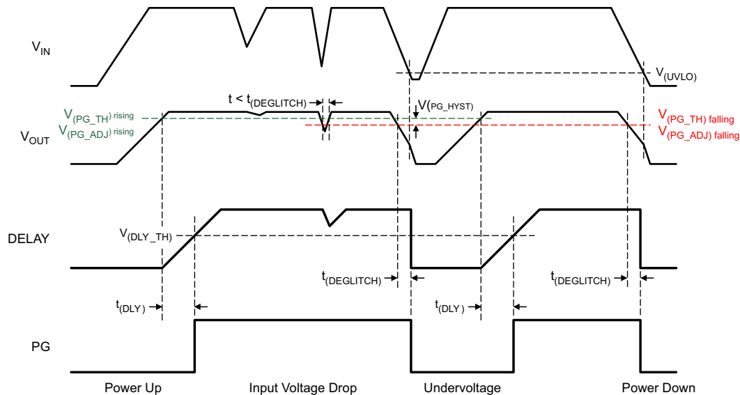
FIG 22. Power-Up and Conditions for Activation of Power Good
