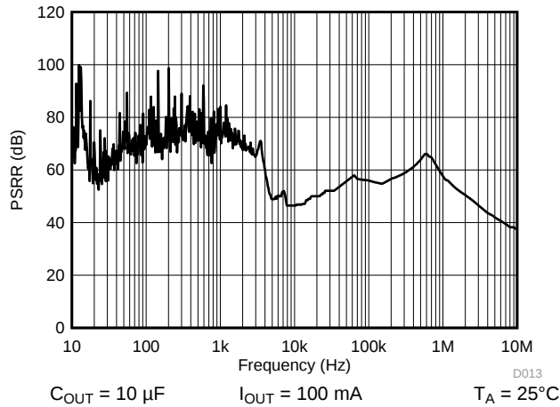
FIG 13. PSRR vs Frequency
