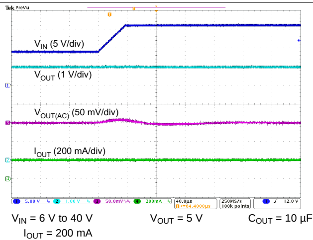
FIG 17. Line Transient
