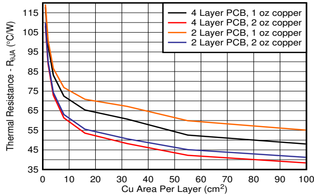
7-4. R_{\theta JA} vs Copper Area 2s2p DCY Package
