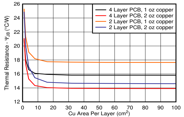
7-3. \psi_{JB} vs Copper Area 2s2p DRB Package
