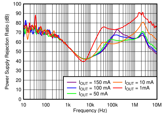
Figure 7-9. PSRR
