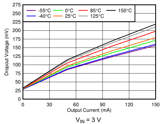
図 5-8. Dropout Voltage ( V_{DO} ) vs I_{OUT}
