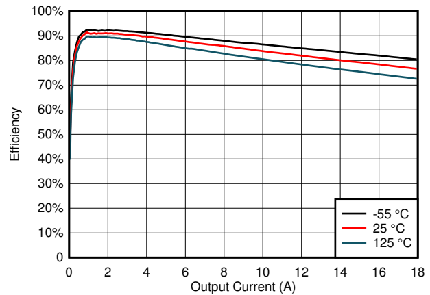
7-26. Efficiency for VIN = 5 V, VOUT = 1.5 V at 500-kHz Switching Frequency
