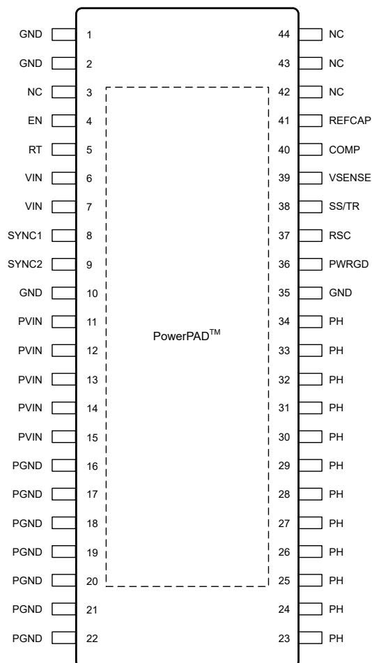
6-2. DDW Package 44-Pin HTSSOP Top View
