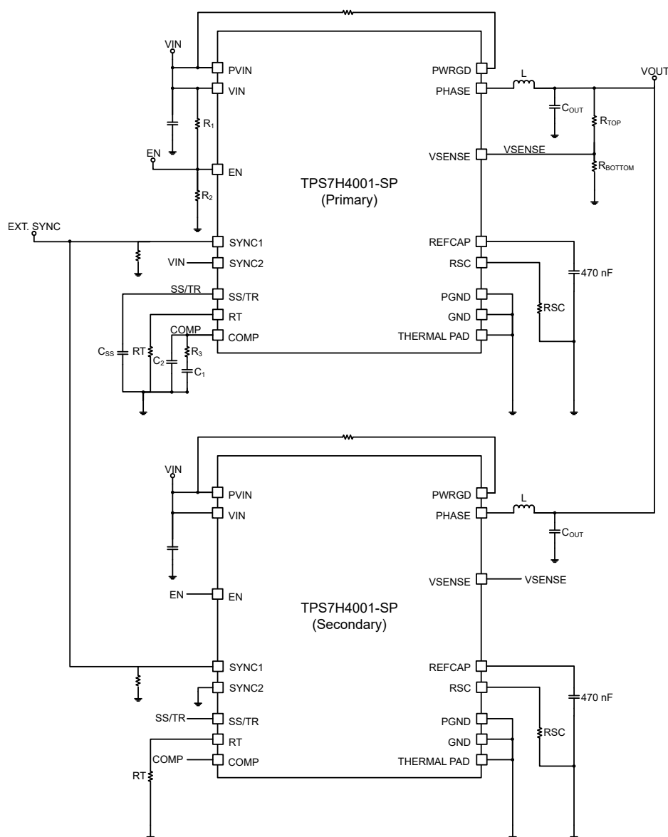
9-3. Parallel Configuration With External Sync
