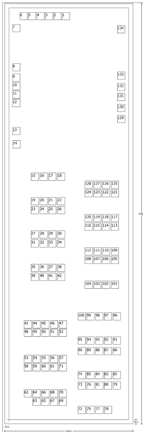
図 6-3. TPS7H4001-SP Bare Die Diagram
