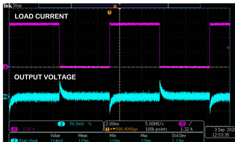
Figure 8-3. 3-A Step Response for 500-kHz Switching Operation
