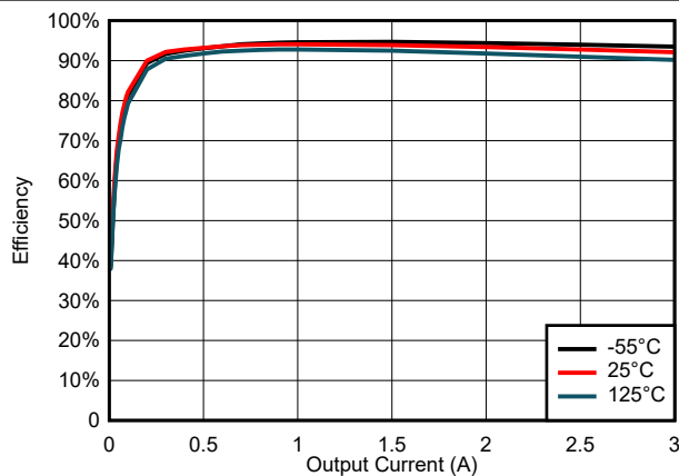
VOUT = 2.5 V, f_{\text{sw}} = 500\ \text{kHz}
