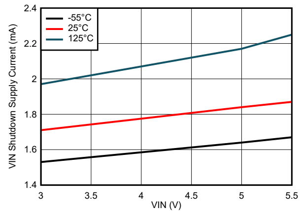
FIG 6-4. VIN Shutdown Supply Current Variation
