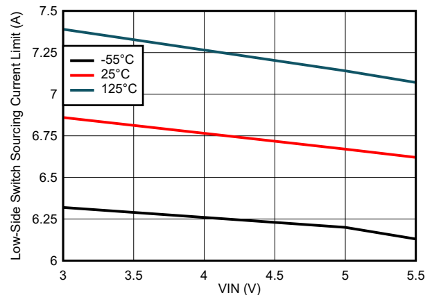
6-12. Low-Side Switch Sourcing Current Limit Variation
