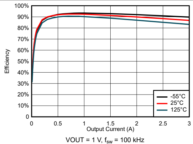
FIG 6-46. Efficiency for V_{\text{IN}} = 5.5\ \text{V}
