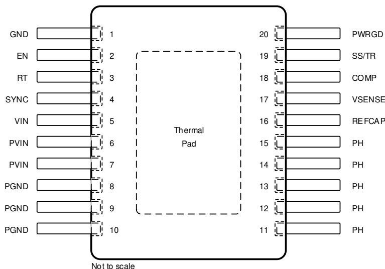
図 5-1. HKH Package 20-Pin CFP Bottom View
