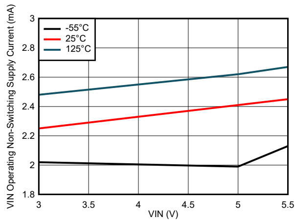
FIG 6-3. VIN Operating Non-Switching Supply Current Variation
