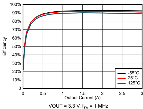
FIG 6-45. Efficiency for V_{\text{IN}} = 5\ \text{V}
