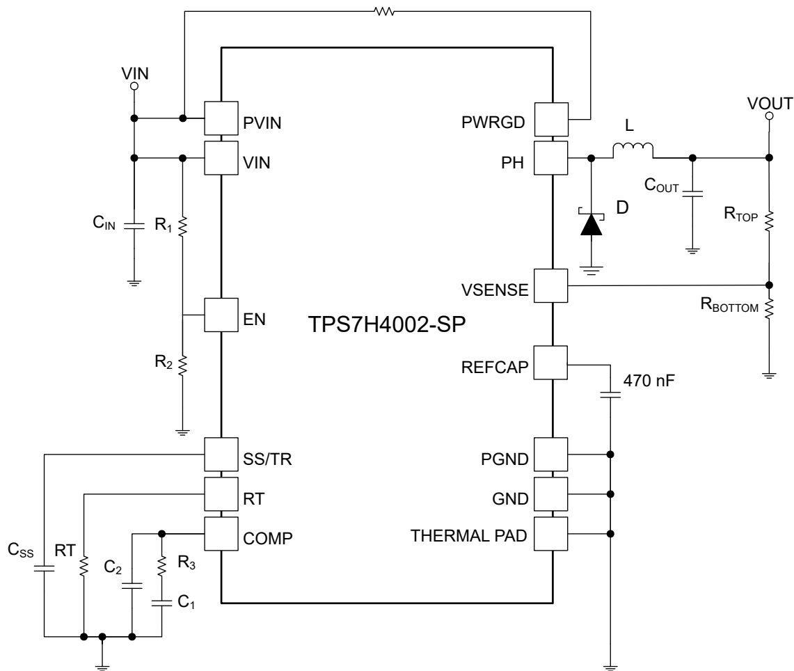
図 8-1. Typical Application Schematic
