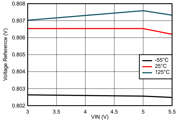
FIG 6-1. Voltage Reference Variation
