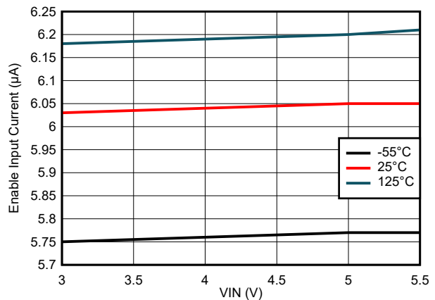
FIG 6-6. Enable Input Current Variation
