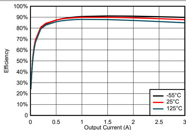
图 6-49. Efficiency fo V_{\text{IN}} = 5.5\ \text{V}
