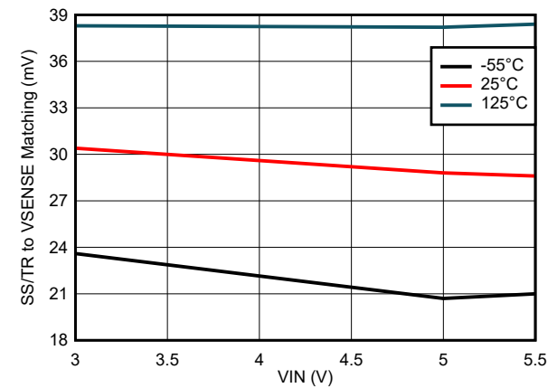
6-10. SS/TR to VSENSE Matching Variation
