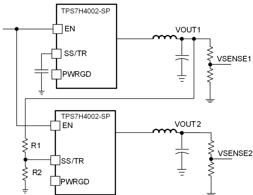
FIG 7-7. Ratiometric and Simultaneous Start-Up Sequence
