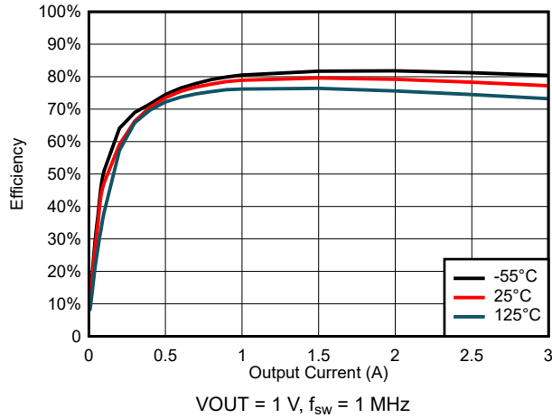
FIG 6-41. Efficiency for V_{\text{IN}} = 5\ \text{V}
