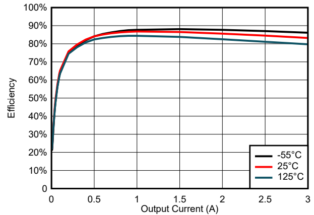
VOUT = 1 V, f_{\text{sw}} = 500\ \text{kHz}
