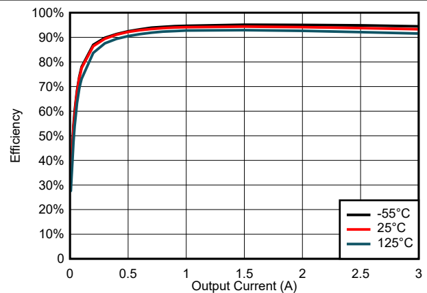
VOUT = 3.3 V, f_{\text{sw}} = 500\ \text{kHz}
