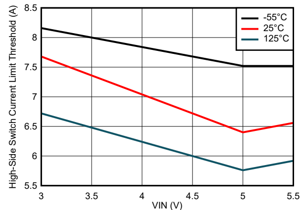
6-11. High-Side Switch Current Limit Threshold Variation
