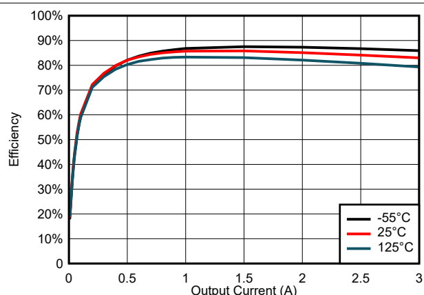
图 6-48. Efficiency for V_{\text{IN}} = 5.5\ \text{V}
