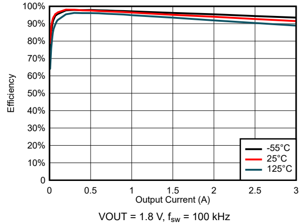
Figure 6-18. Efficiency for V_{\text{IN}} = 3\ \text{V}
