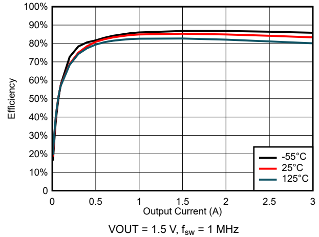
FIG 6-42. Efficiency for V_{\text{IN}} = 5\ \text{V}
