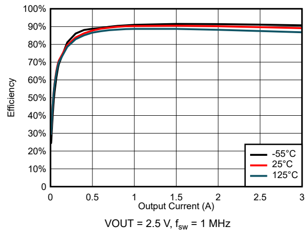
FIG 6-44. Efficiency for V_{\text{IN}} = 5\ \text{V}
