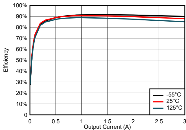
VOUT = 1.5 V, f_{\text{sw}} = 500\ \text{kHz}
