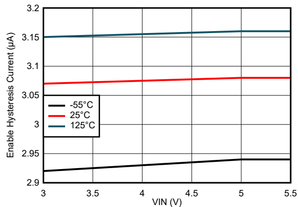
FIG 6-5. Enable Hysteresis Current Variation
