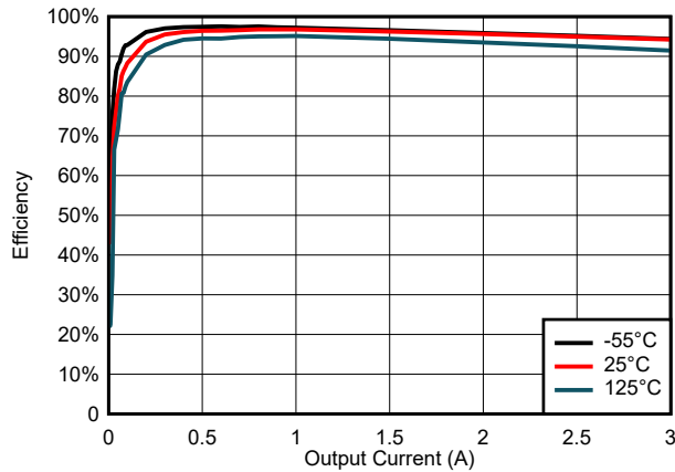
VOUT = 3.3 V, f_{\text{sw}} = 100\ \text{kHz}
