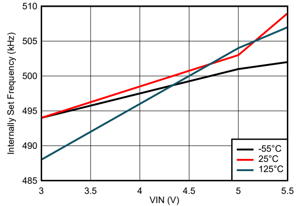
FIG 6-2. Internally Set Frequency Variation
