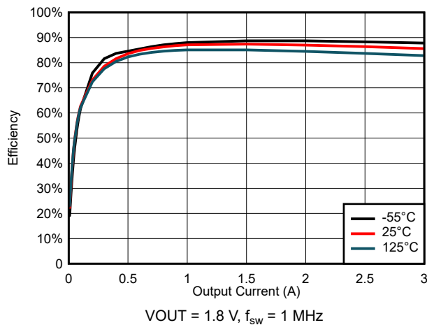
FIG 6-43. Efficiency for V_{\text{IN}} = 5\ \text{V}
