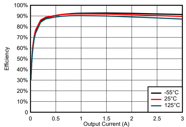
VOUT = 1.8 V, f_{\text{sw}} = 500\ \text{kHz}
