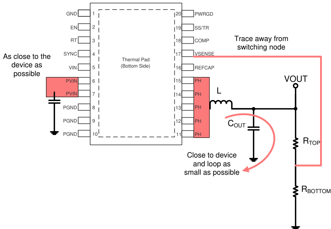
10-1. PCB Layout Example
