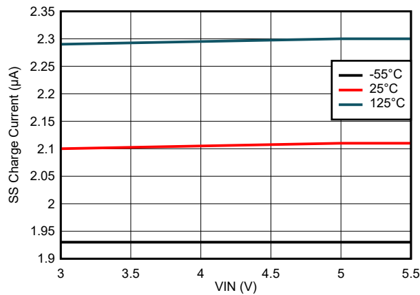
6-9. SS Charge Current Variation
