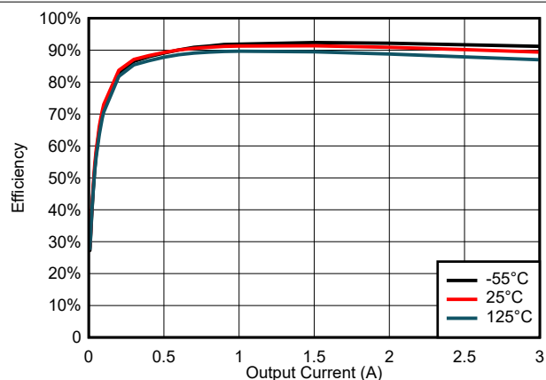
图 6-50. Efficiency for V_{\text{IN}} = 5.5\ \text{V}
