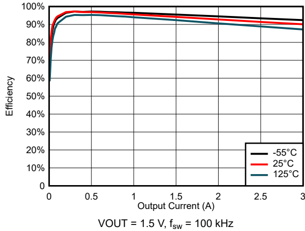
Figure 6-17. Efficiency for V_{\text{IN}} = 3\ \text{V}
