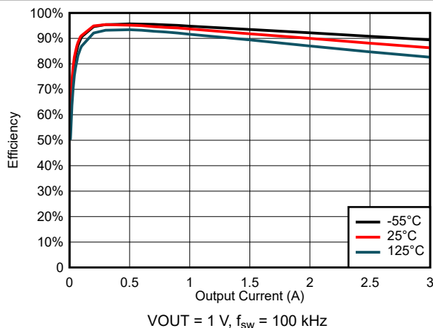
Figure 6-16. Efficiency for V_{\text{IN}} = 3\ \text{V}
