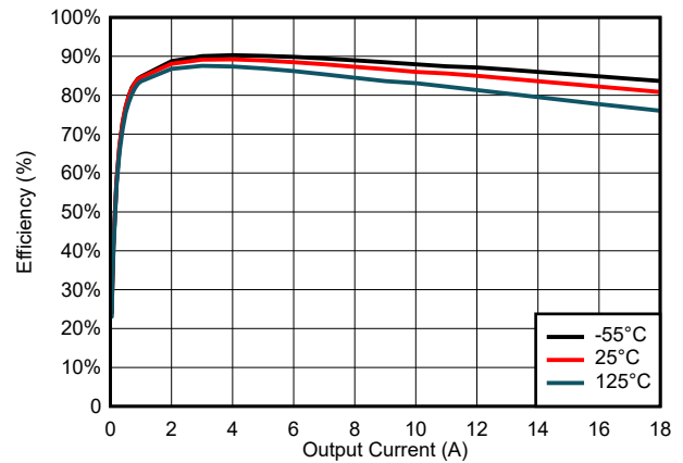
6-32. Efficiency for VIN = 7 V
