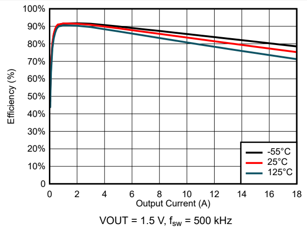
6-22. Efficiency for VIN = 3 V
