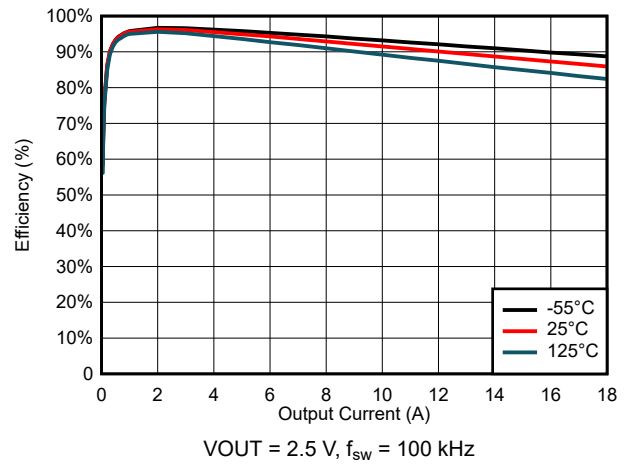
6-20. Efficiency for V_{IN} = 5 \text{ V}
