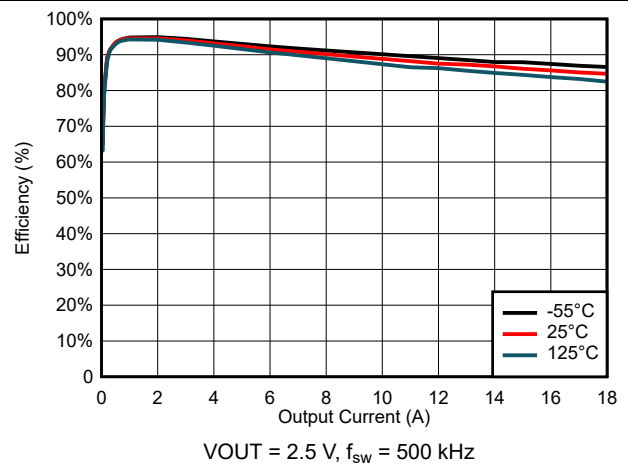
6-24. Efficiency for V_{IN} = 3 \text{ V}
