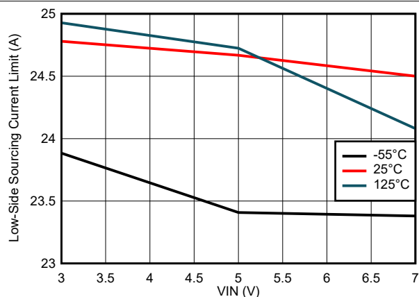
Figure 6-13. Low-Side Sourcing Current Limit Variation
