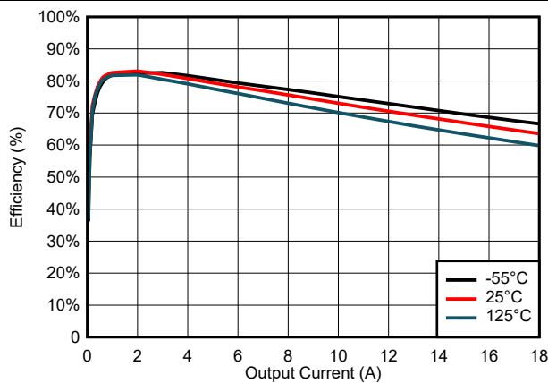
6-33. Efficiency for VIN = 7 V
