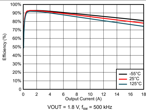
6-23. Efficiency for V_{IN} = 3 \text{ V}
