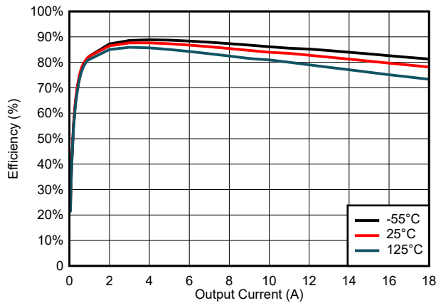
6-31. Efficiency for VIN = 7 V
