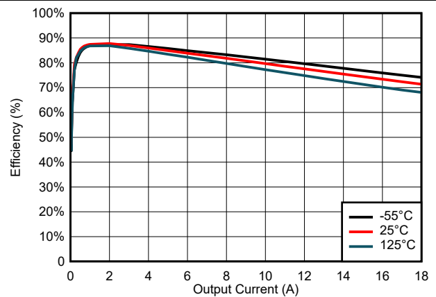
6-34. Efficiency for VIN = 7 V
