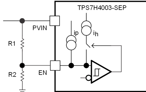
7-2. Adjustable PVIN UVLO
