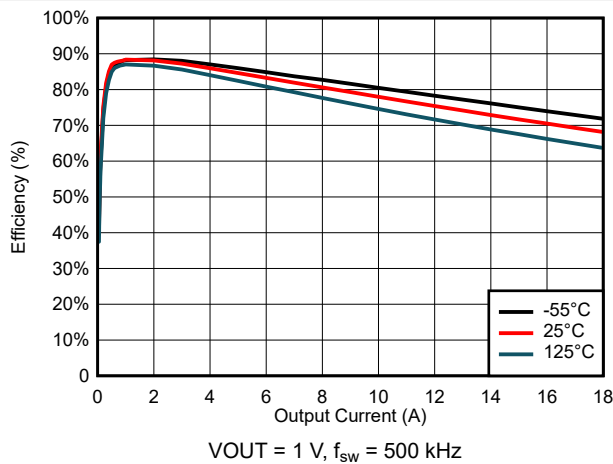
6-21. Efficiency for V_{IN} = 3 \text{ V}
