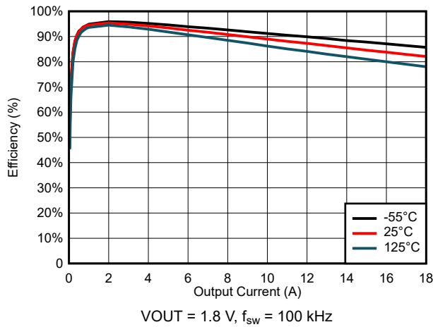
6-19. Efficiency for V_{IN} = 5 \text{ V}
