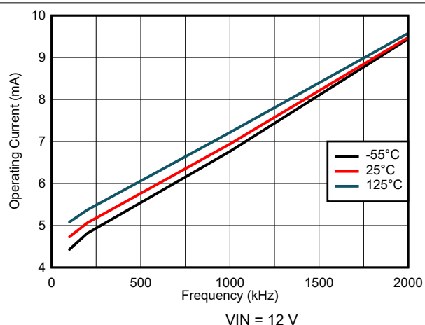
図 7-2. Operating Current Variation
