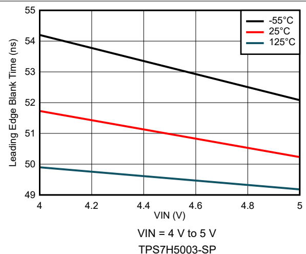
7-39. Leading Edge Blank Time Variation
