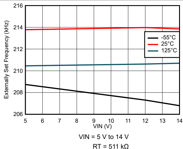
7-22. Externally Set Frequency Variation
