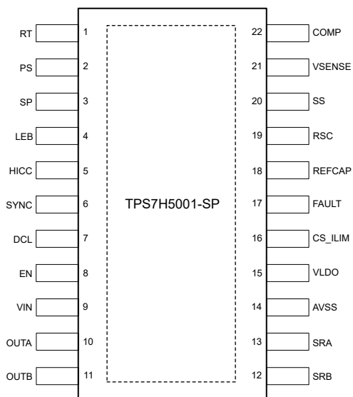
図 6-1. TPS7H5001-SP HFT Package 22-Pin CFP With Thermal Pad (Top View)
