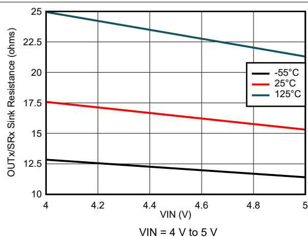
Figure 7-63. Output Sink Resistance Variation
