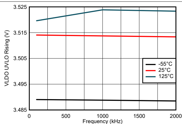
図 7-5. VLDO UVLO Rising Variation
