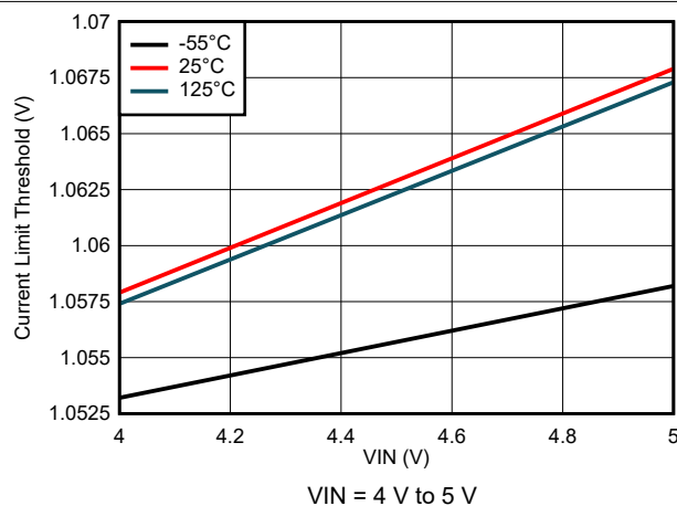
図 7-17. Current Limit Threshold Variation
