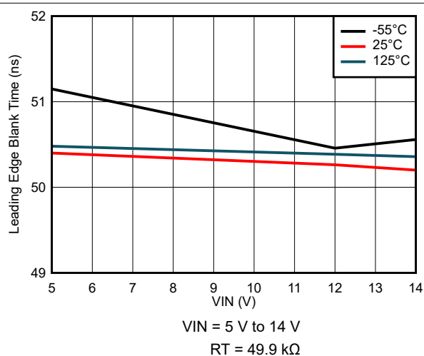
7-36. Leading Edge Blank Time Variation
