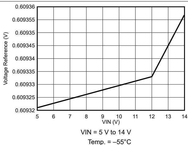
Figure 7-12. Voltage Reference Variation
