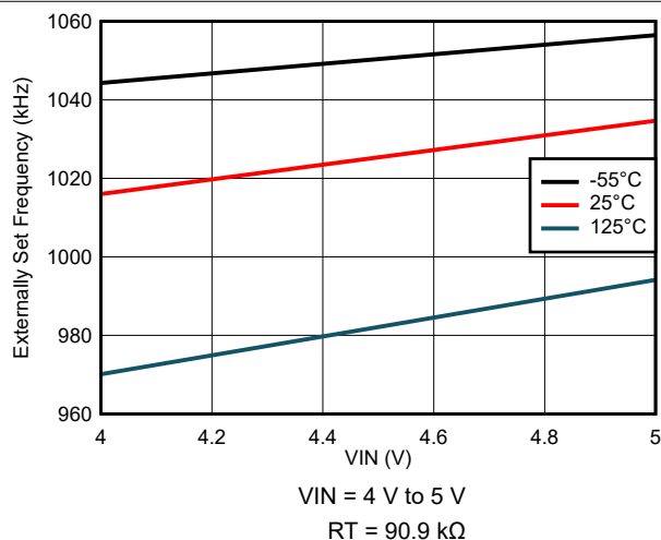
7-23. Externally Set Frequency Variation
