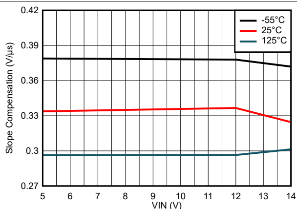
7-68. Slope Compensation Variation
