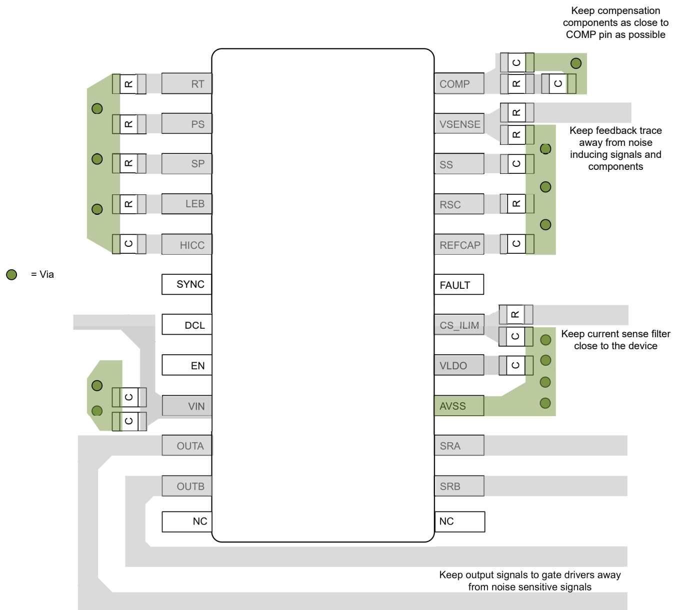
図 9-5. PCB Layout Example for TSSOP Package
