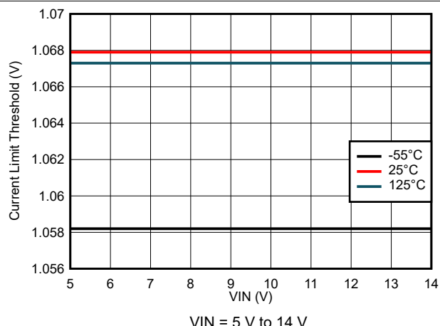
図 7-18. Current Limit Threshold Variation
