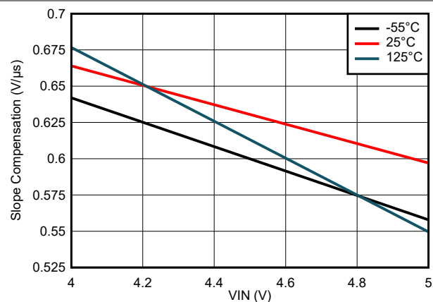
7-69. Slope Compensation Variation
