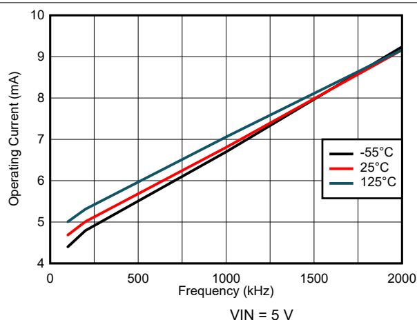
図 7-1. Operating Current Variation
