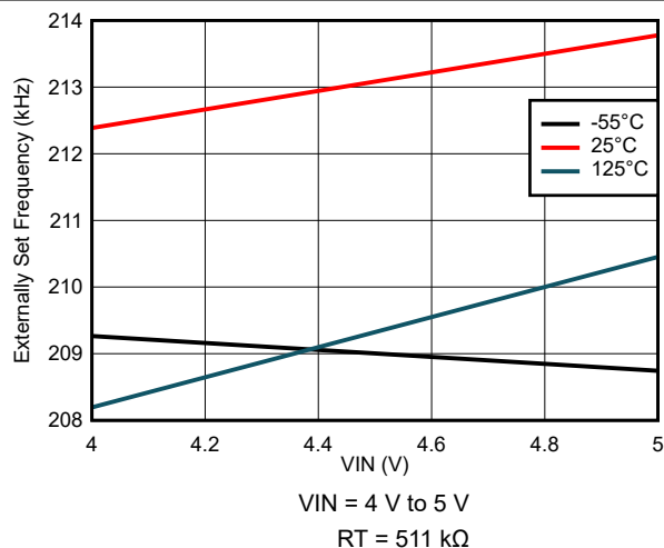
7-21. Externally Set Frequency Variation
