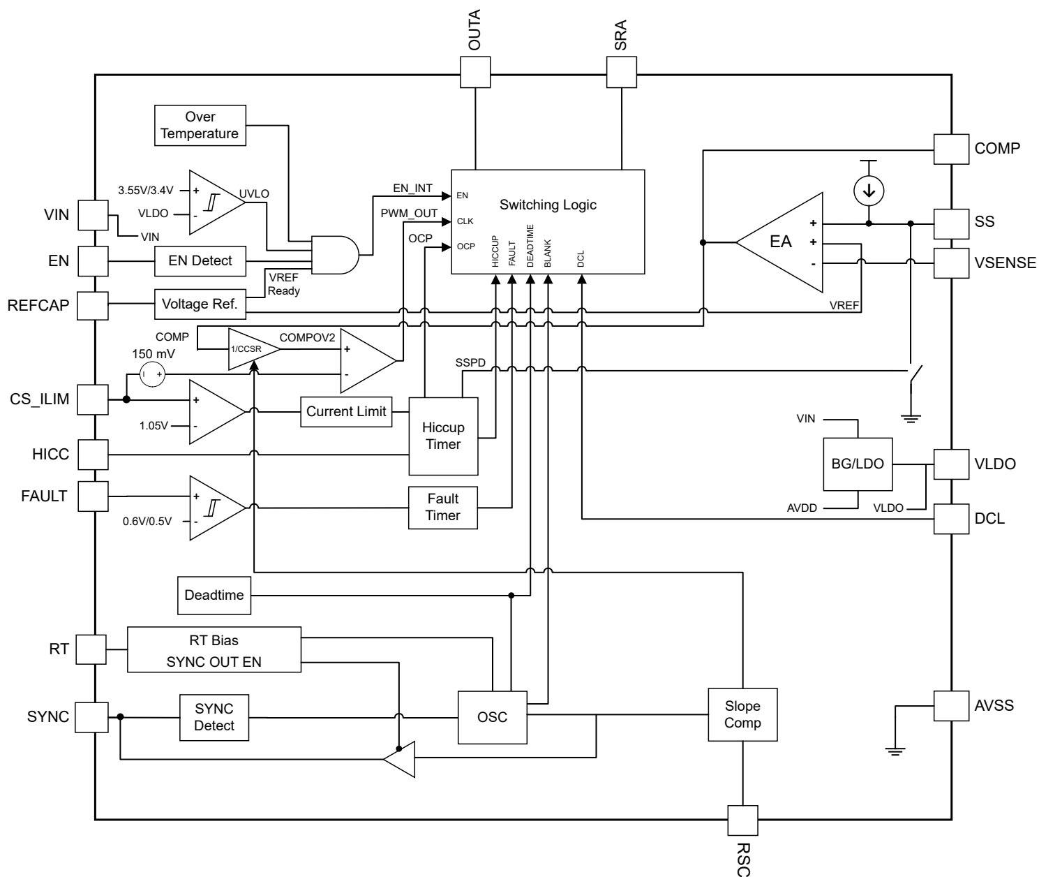
図 8-3. TPS7H5003-SP Functional Block Diagram
