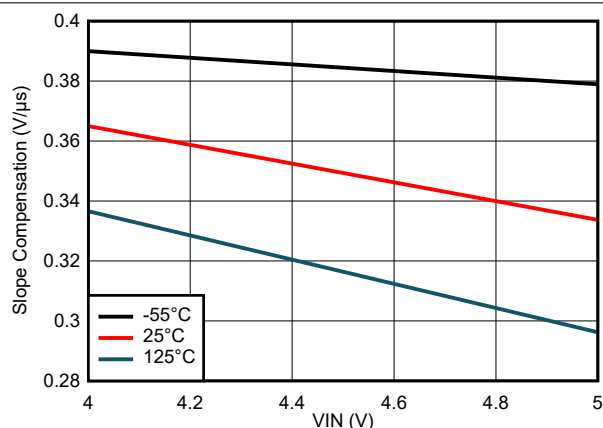
7-67. Slope Compensation Variation
