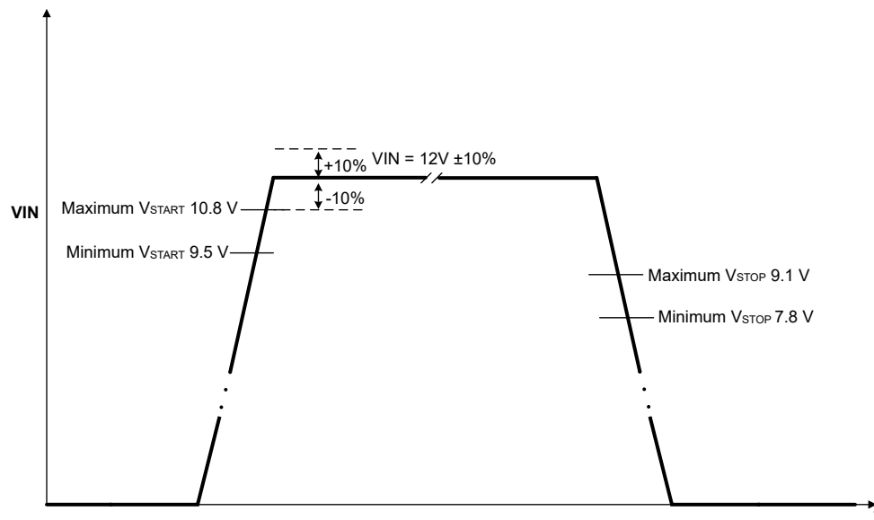
図 8-6. Start-Up and UVLO Values for Two-Resistor Configuration With VIN = 12 V
