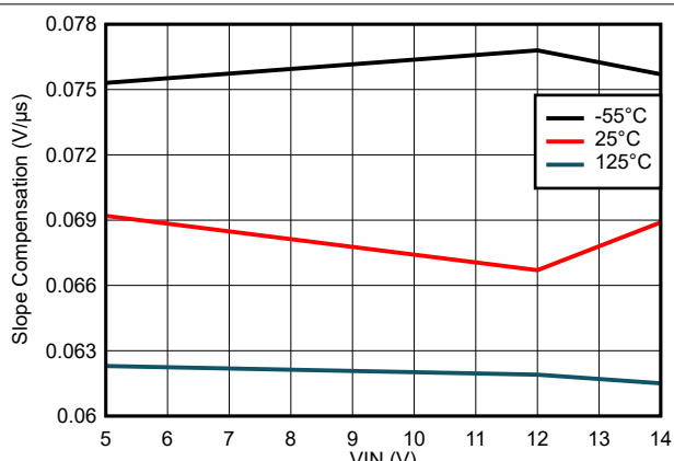
7-68. Slope Compensation Variation
