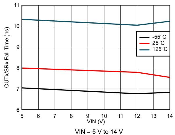
Figure 7-60. Output Fall Time Variation
