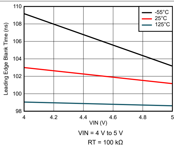
7-37. Leading Edge Blank Time Variation
