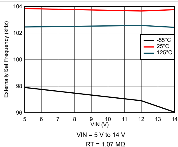
7-20. Externally Set Frequency Variation
