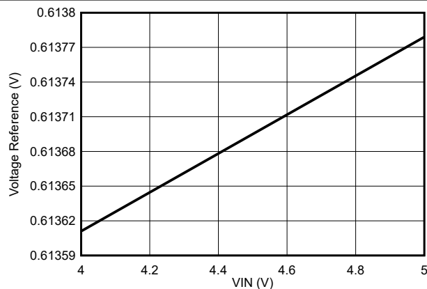
図 7-13. Voltage Reference Variation
