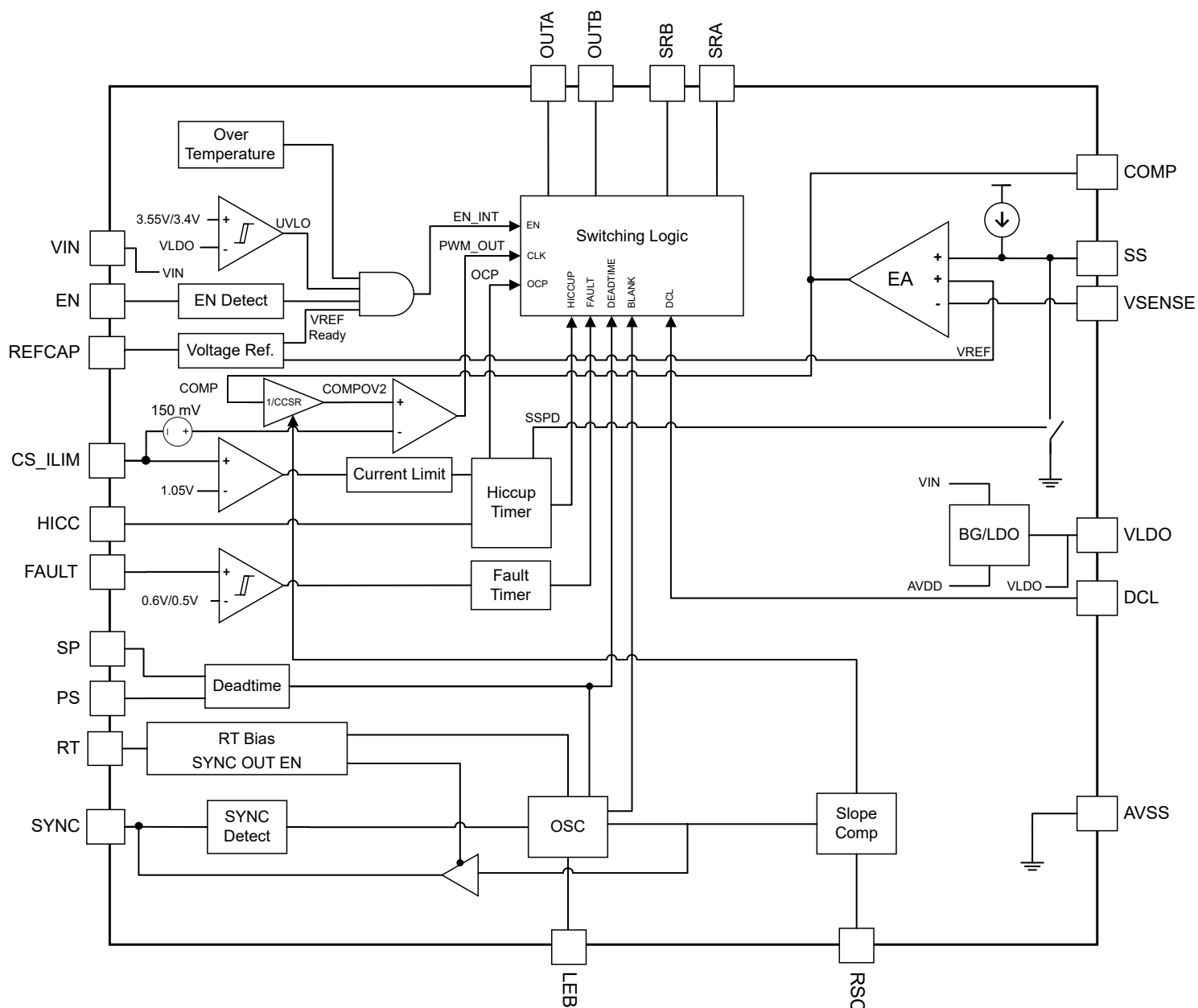
図 8-1. TPS7H5001-SP Functional Block Diagram
