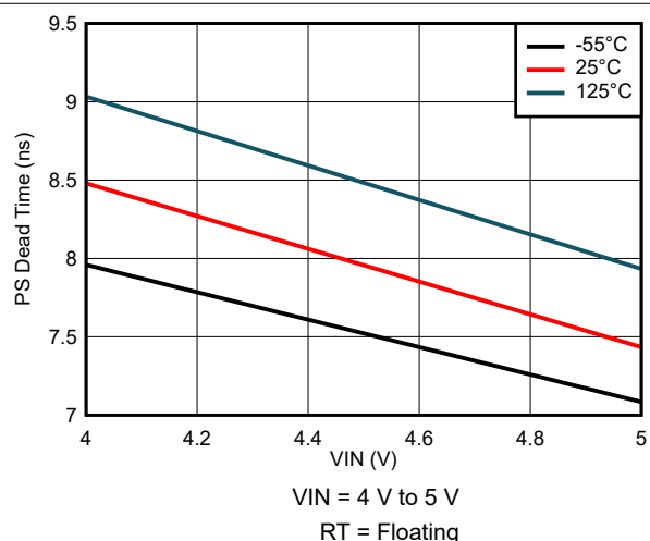
7-41. PS Dead Time Variation
