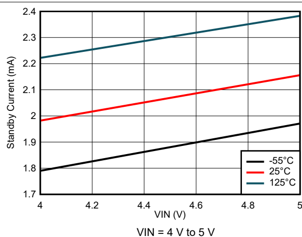
図 7-3. Standby Current Variation
