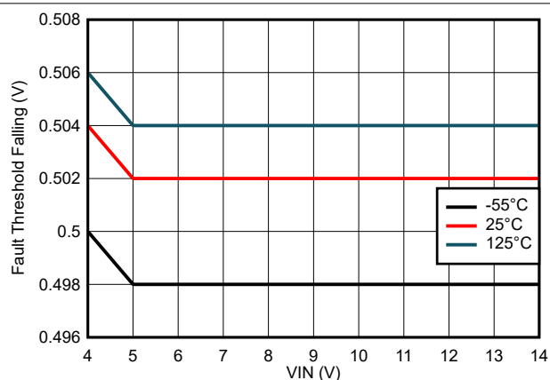
7-32. FAULT Threshold Falling Variation
