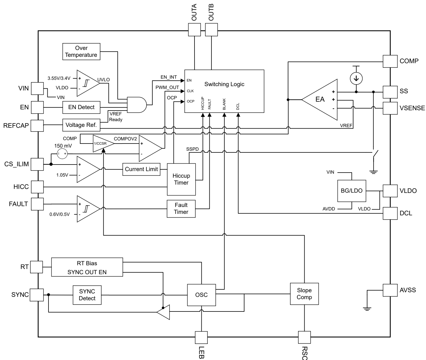
図 8-4. TPS7H5004-SP Functional Block Diagram
