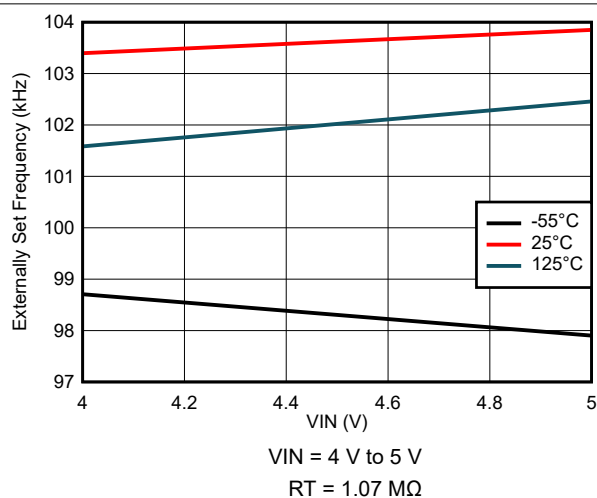
7-19. Externally Set Frequency Variation
