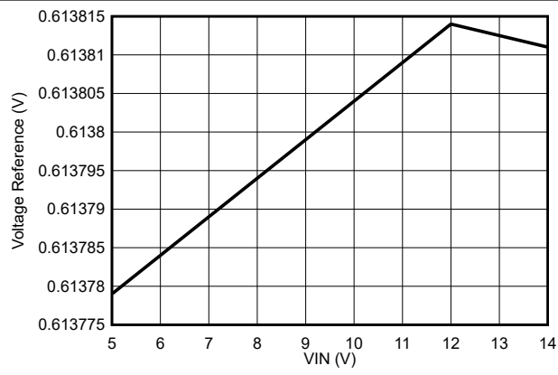
図 7-14. Voltage Reference Variation
