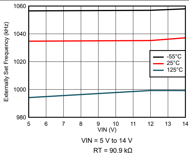
7-24. Externally Set Frequency Variation
