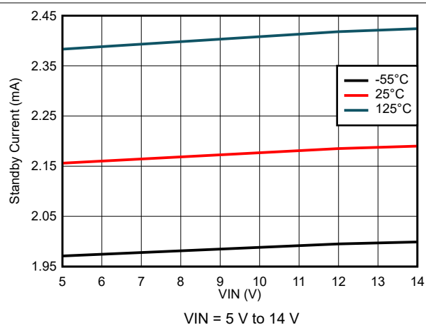
図 7-4. Standby Current Variation
