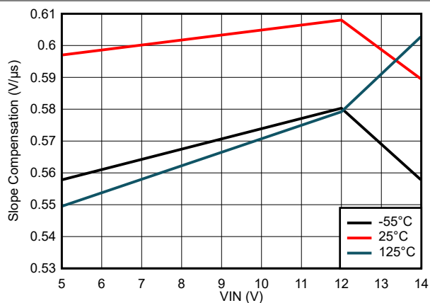
7-70. Slope Compensation Variation
