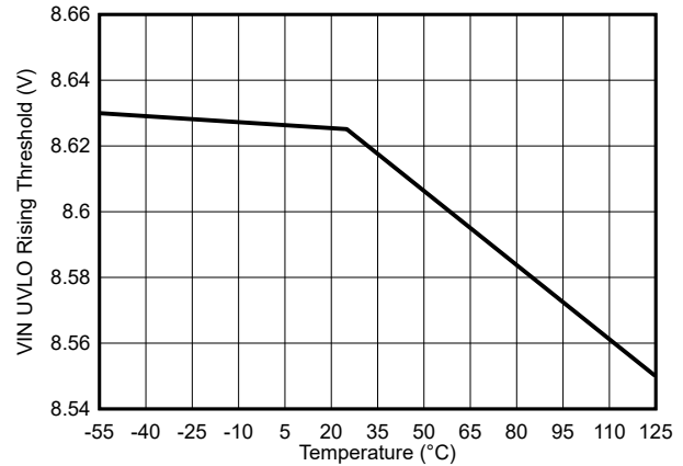
Figure 7-26. VIN UVLO Rising Threshold vs Temperature
