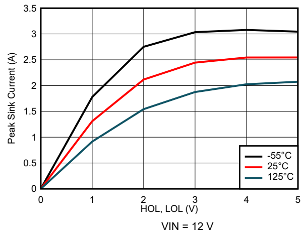
Figure 7-12. Peak Sink Current vs Output Voltage
