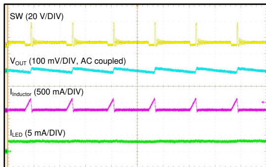
8-8. Switching-Dimming Duty = 10%
