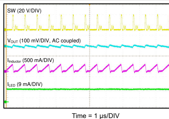
Figure 8-7. Switching-Dimming Duty = 50%
