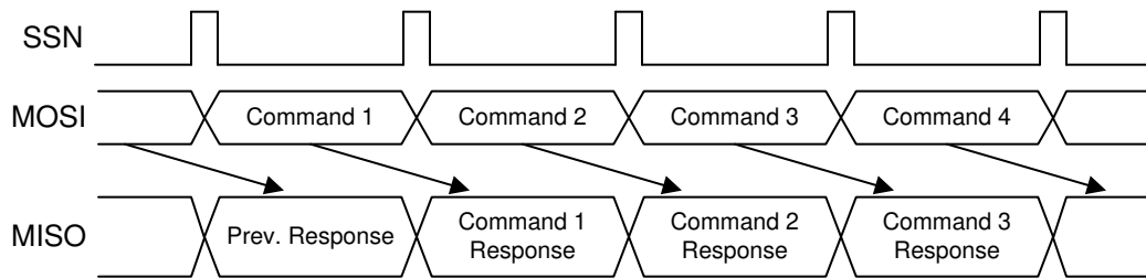
FIG 7-15. SPI Command and Response Sequence
