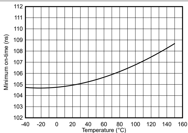
FIG 6-17. Minimum On-time vs Temperature
