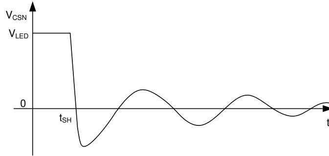
FIG 7-8. Short Circuit Fault Transient Behavior
