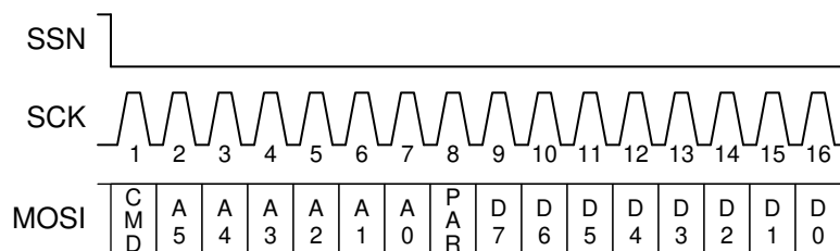
FIG 7-16. Command Frame Format
