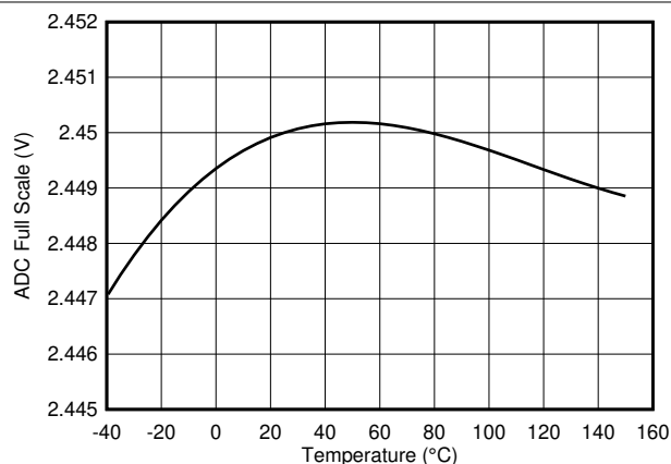
FIG 6-15. ADC Full Scale vs Temperature
