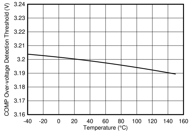
FIG 6-20. COMP Overvoltage Detection Threshold vs Temperature
