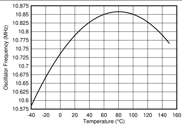
FIG 6-14. Oscillator Frequency vs Temperature
