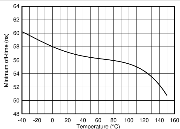
FIG 6-18. Minimum Off-time vs Temperature
