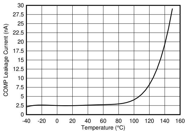
FIG 6-21. COMP Leakage Current vs Temperature
