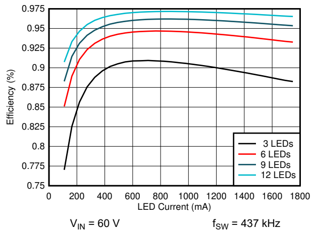
FIG 6-22. Efficiency vs LED Current
