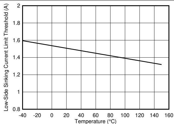
FIG 6-13. Low-Side Sinking Current Limit Threshold vs Temperature
