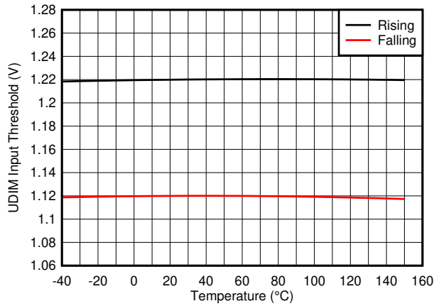
FIG 6-19. UDIM Input Threshold vs Temperature
