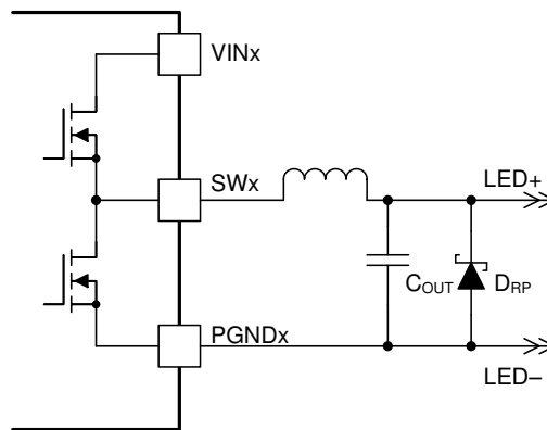
FIG 7-9. CSP and CSN Transient Protection Using an External Diode
