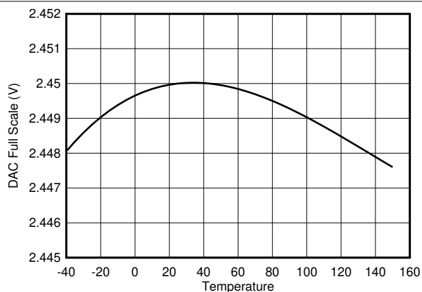
FIG 6-16. DAC Full Scale vs Temperature
