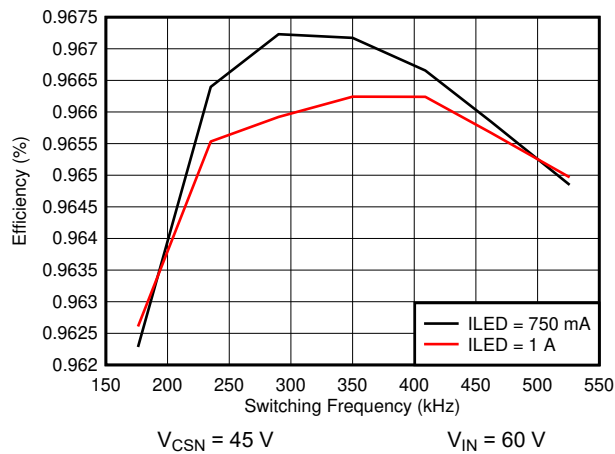
FIG 6-23. Efficiency vs Switching Frequency
