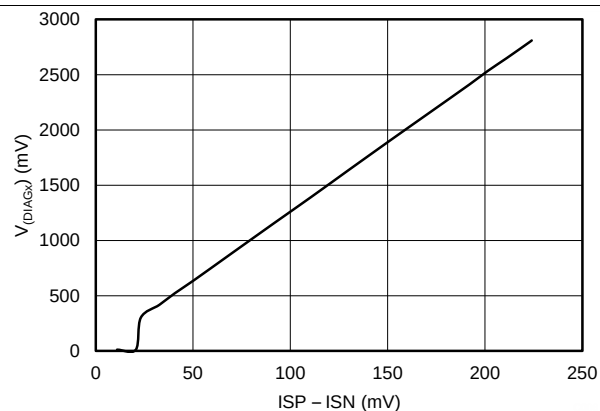
Figure 6. V_{(\text{DIAGx})} vs V_{(\text{ISP} - \text{ISN})}
