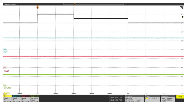
FIG 6-19. Transient Overvoltage
