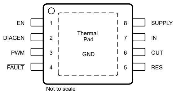
図 5-1. DGN Package 8-Pin HVSSOP With PowerPAD™ Integrated Circuit Package (Top View)
