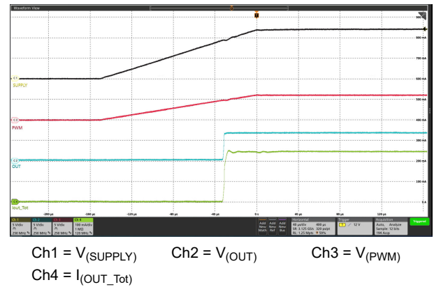
Figure 6-10. Power-Up Sequence
