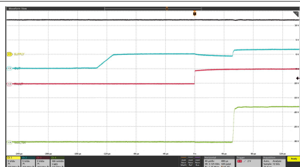
图 6-15. LED Open Protection Recovery
