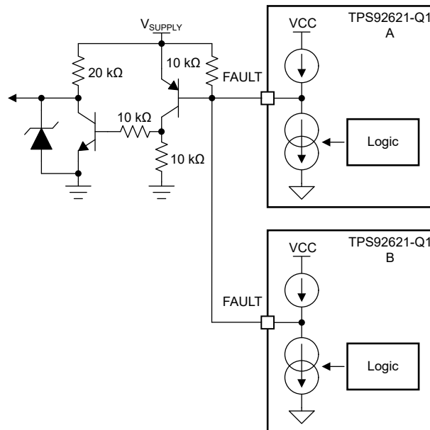
FIG 7-7. FAULT Bus for One-Fails-Others-On Application
