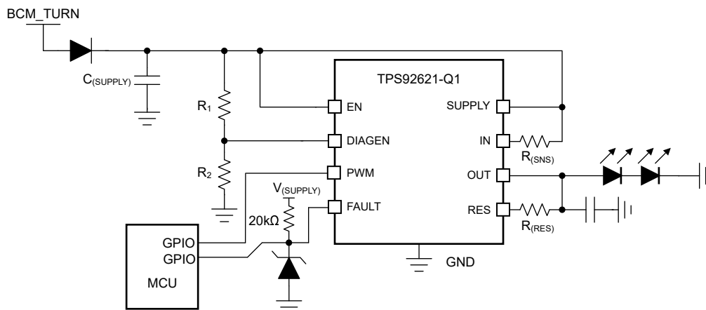
8-4. Typical Application Schematic
