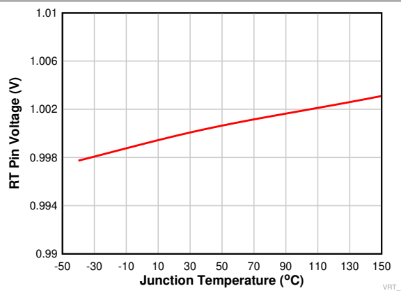
6-6. RT Pin Voltage vs Junction Temperature
