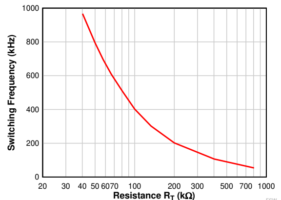
6-22. Channel Switching Frequency F_{SW} vs R_T Resistance
