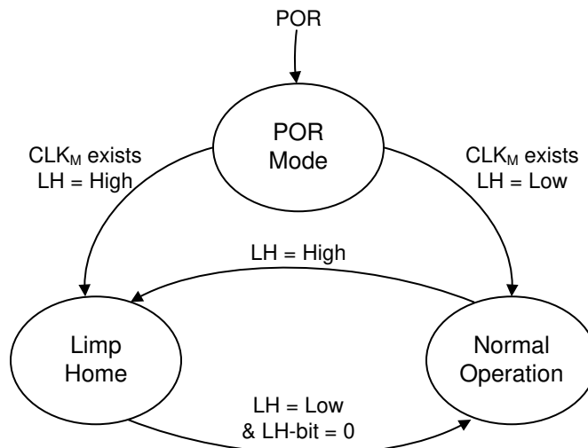
FIG 7-19. TPS92682 Functional Mode
