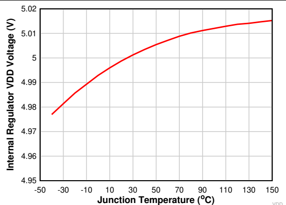
6-2. Regulated VDD Voltage vs Junction Temperature
