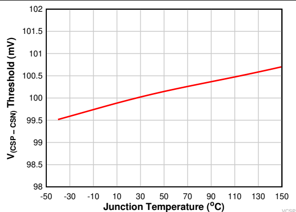
6-20. V_{(CSP - CSN)} Voltage vs Junction Temperature
