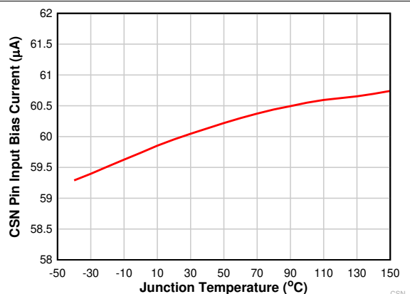
FIG 6-16. CSN Pin Input Bias Current vs Junction Temperature
