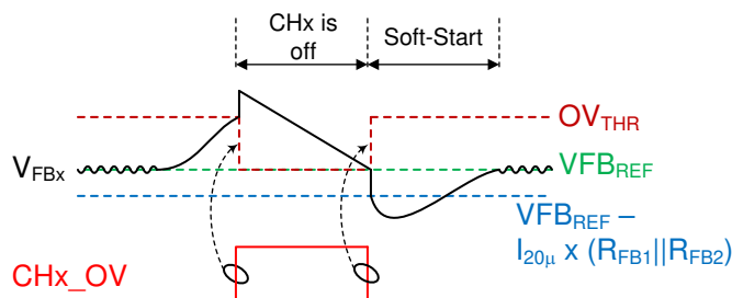
FIG 7-16. Non-latched OV Fault in CV Mode
