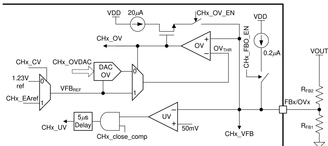
FIG 7-15. OV and UV Faults
