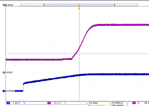
CH1: V_{COMP1} pin CH3: CV Boost V_{OUT}
