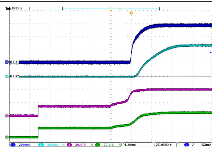
CH1: Boost I_{LED} current CH2: Buck-Boost I_{LED} current CH3: Boost LED+ voltage (12×LED) CH4: Buck-Boost LED+ voltage (6×LED)
