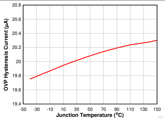
FIG 6-14. OVP Hysteresis Current vs Junction Temperature
