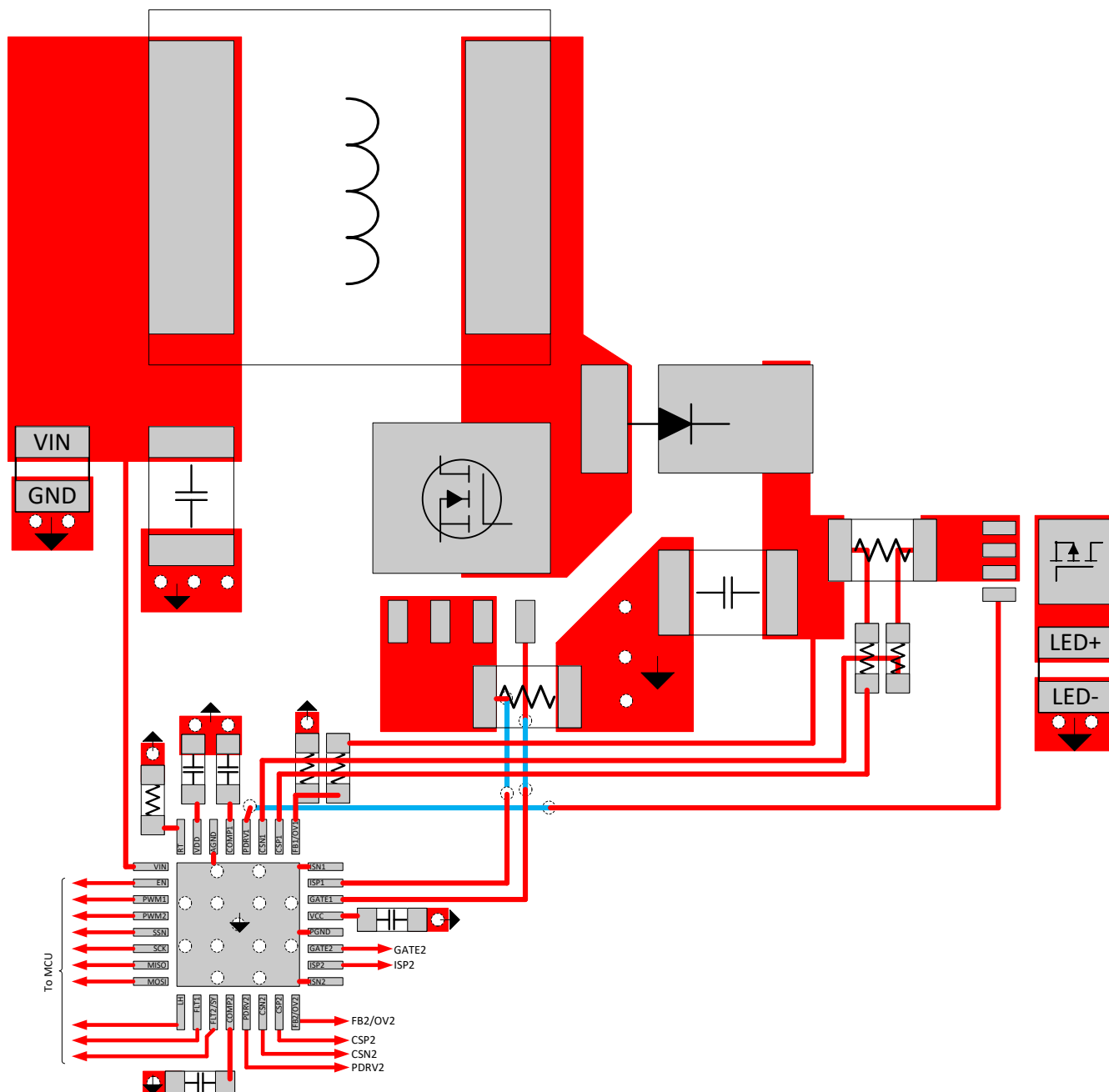
10-1. CC Boost Layout Example
