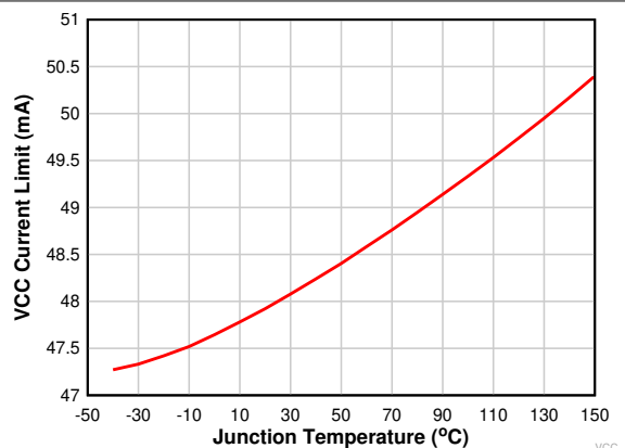
6-4. VCC Current Limit vs Junction Temperature
