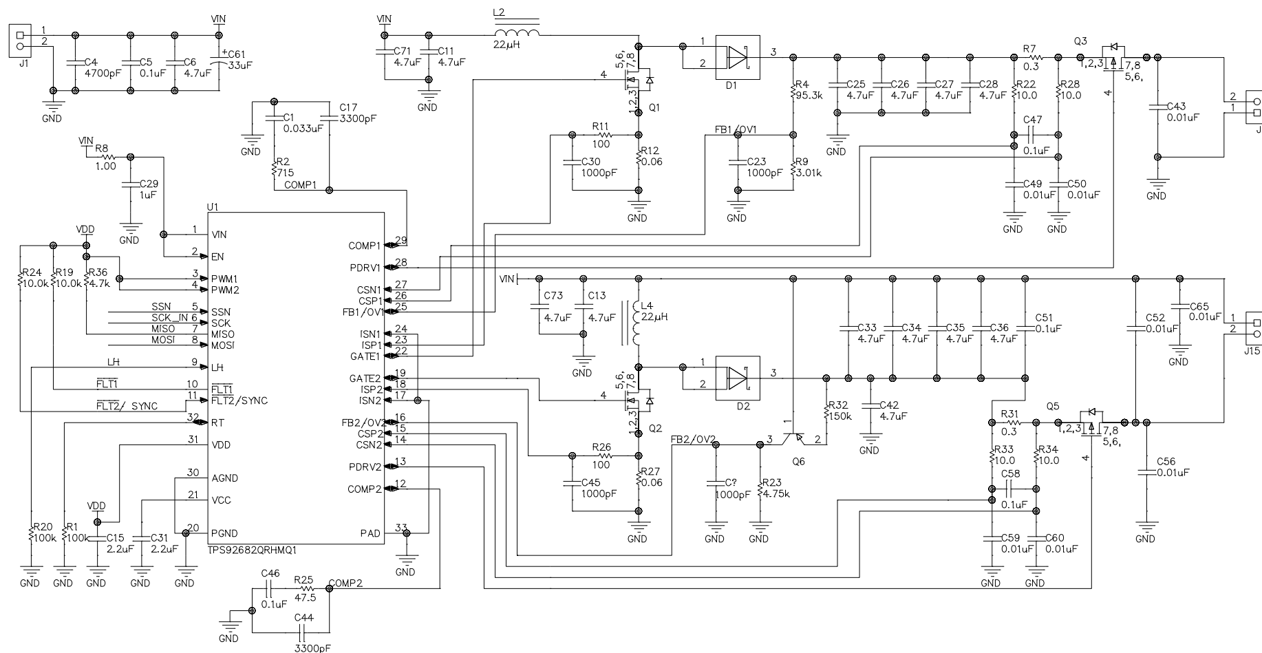
Figure 8-11. CC Mode LED Driver, BOOST, and Buck-Boost
