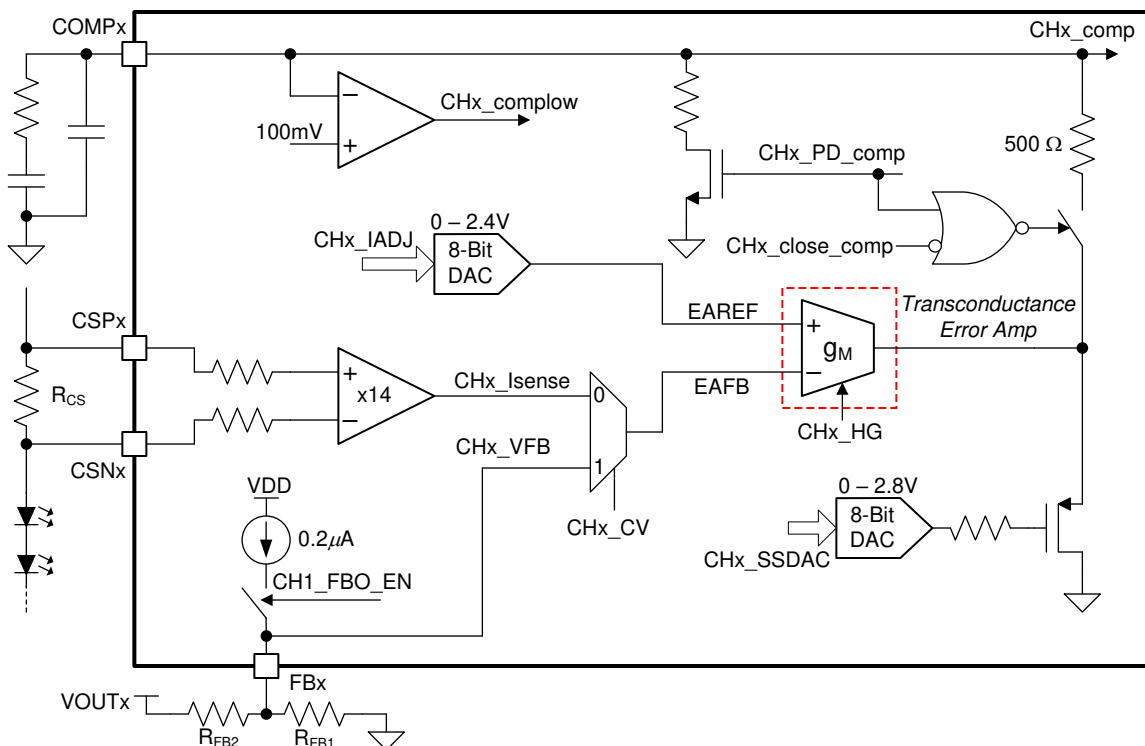
7-8. Feedback Connection to the Error Amplifier
