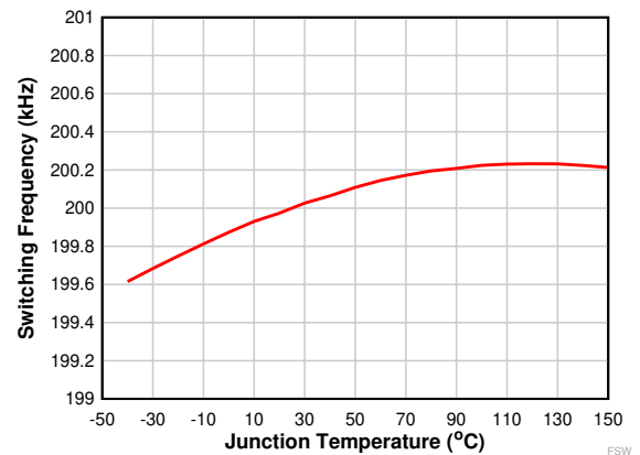
6-8. Switching Frequency vs Junction Temperature
