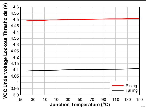
6-5. VCC UVLO Threshold vs Junction Temperature
