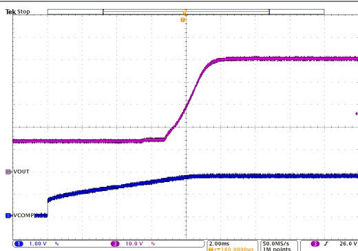
CH1: V_{COMP1} pin CH3: CV Boost V_{OUT}
