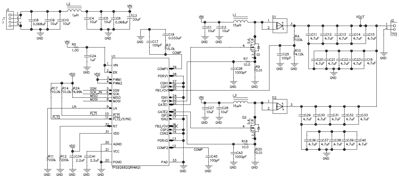
8-24. CV Mode Two-Phase BOOST
