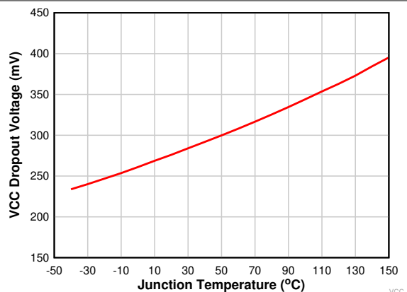
6-3. VCC Dropout Voltage vs Junction Temperature
