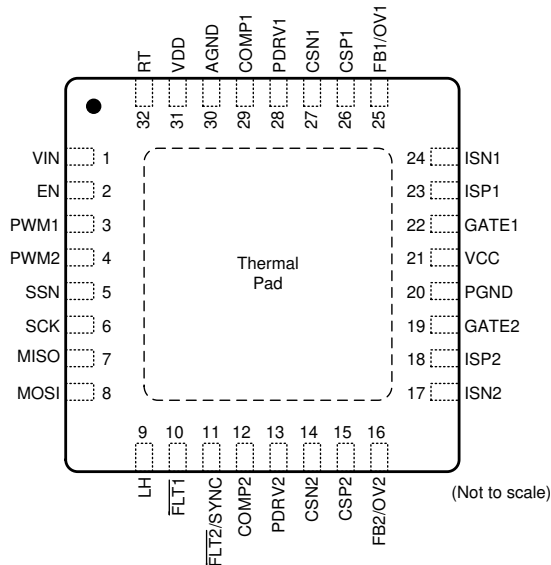
5-1. RHM/RHB Package 32-Pin VQFN with PowerPAD Top View
