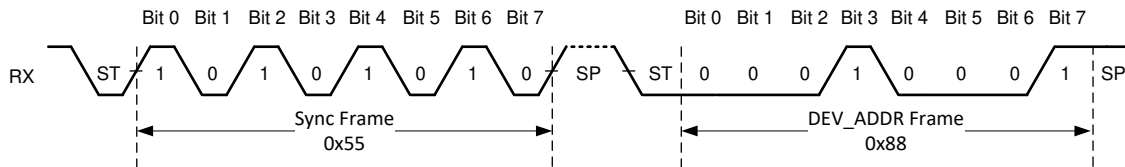
Figure 8-13. Synchronization Byte
