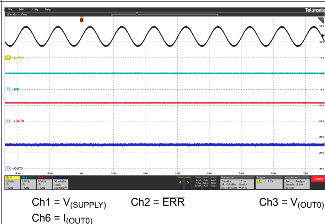
7-18. Superimposed Alternating Voltage 1 kHz
