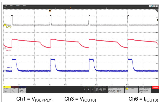
7-13. Supply Dimming In Fail-Safe Mode
