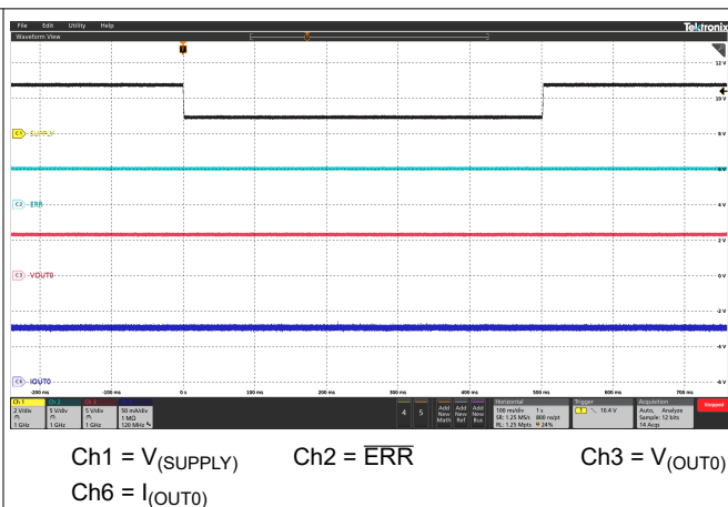
7-14. Transient Undervoltage
