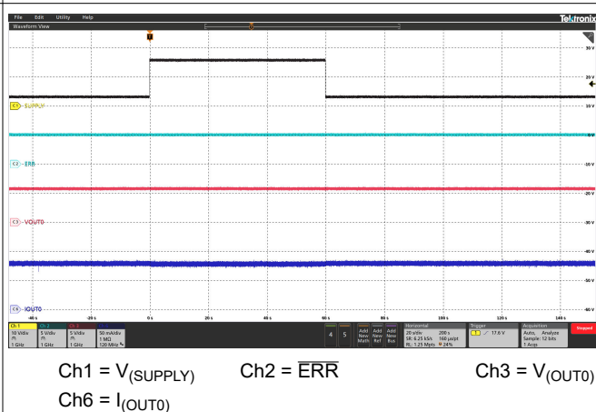
7-16. Jump Start
