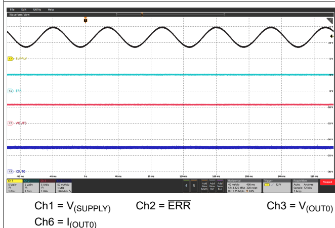
7-17. Superimposed Alternating Voltage 15 Hz
