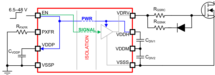
9-2. TPSI3050-Q1 Two-Wire Mode Driving MOSFETs
