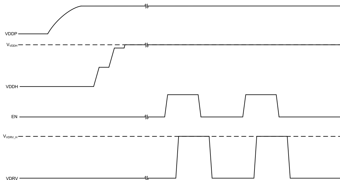
8-2. Three-Wire Mode with TPSI3050-Q1 (Standard Enable)
