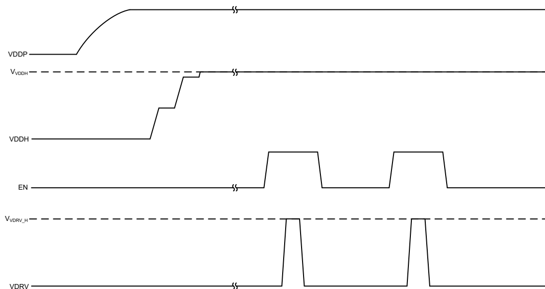
8-3. Three-Wire Mode with TPSI3050S-Q1 (One-shot Enable)
