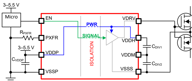
☒ 8-1. Three-Wire Mode Simplified Schematic
