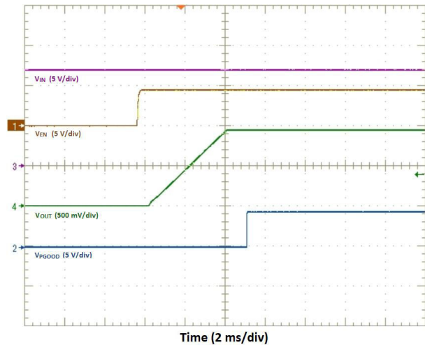
8-3. Start-Up Waveforms
