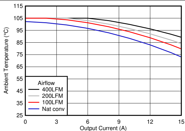
Figure 6-4. Safe Operating Area
