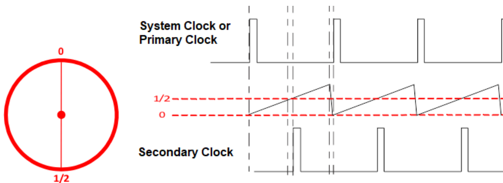
図 7-3. 2-Phase Stackable with 180° Clock Phase Shift
