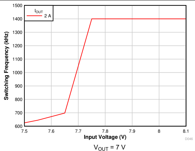
7-12. Frequency Foldback
