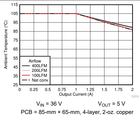
6-22. Safe Operating Area
