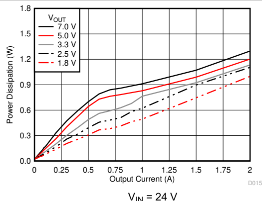
6-13. Power Dissipation versus Output Current
