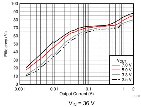
6-18. Efficiency versus Output Current
