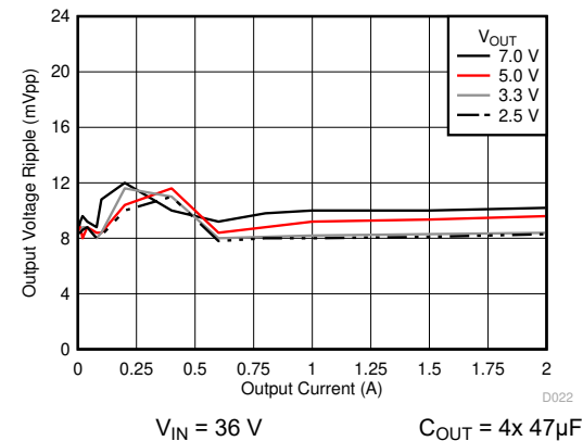
6-20. Voltage Ripple versus Output Current
