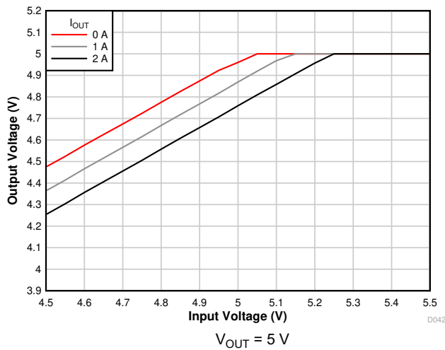
7-9. Voltage Dropout
