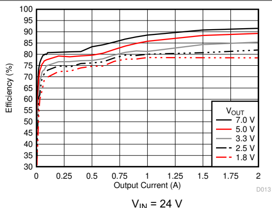
6-11. Efficiency versus Output Current
