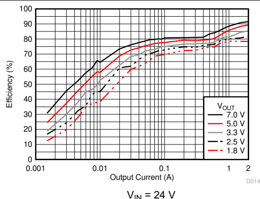
6-12. Efficiency versus Output Current
