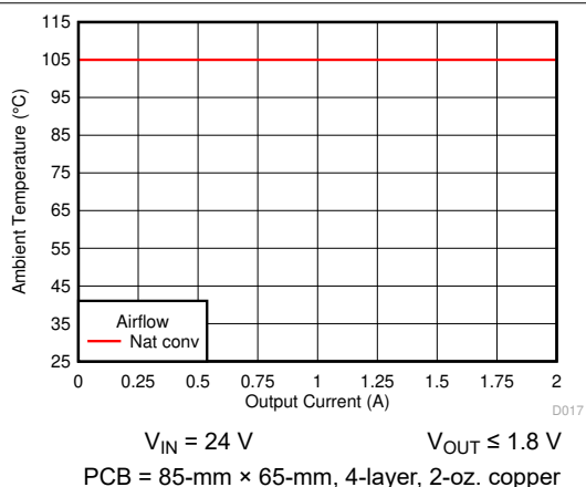
6-15. Safe Operating Area
