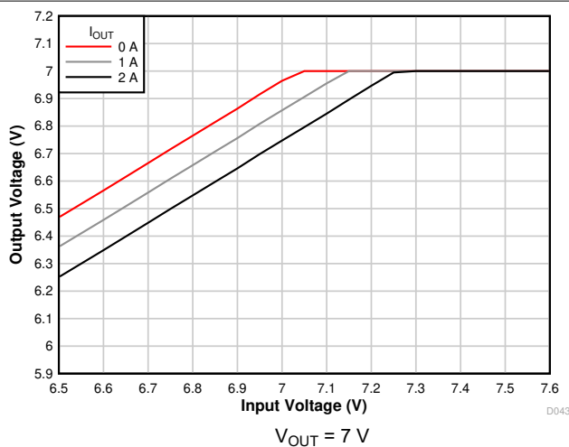
7-11. Voltage Dropout
