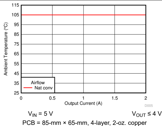
6-5. Safe Operating Area
