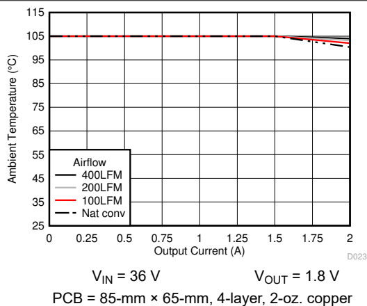
6-21. Safe Operating Area
