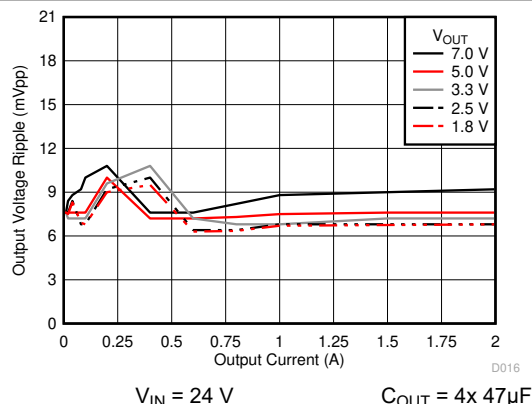
6-14. Voltage Ripple versus Output Current
