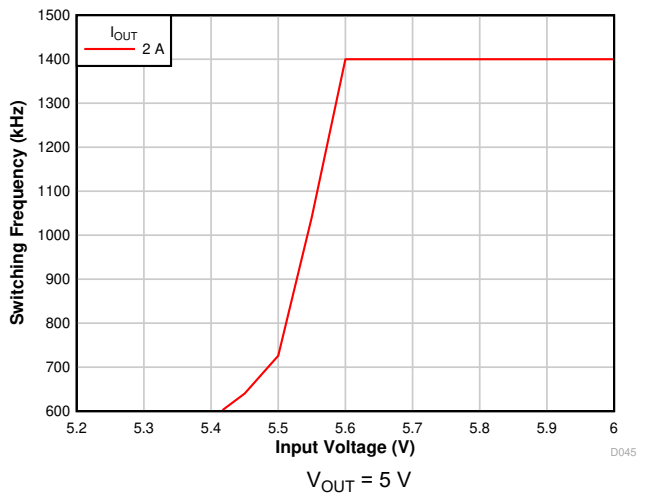
7-10. Frequency Foldback
