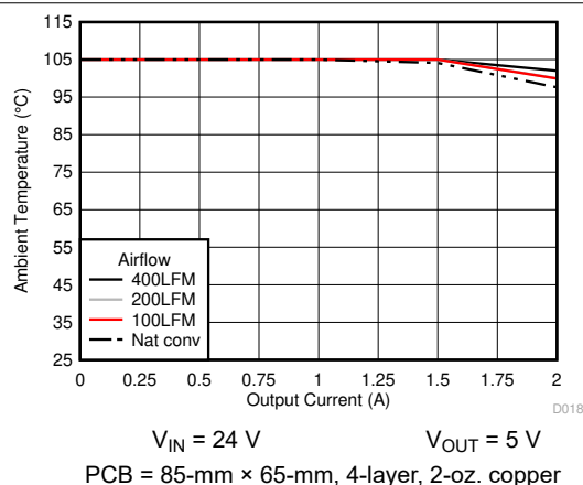
6-16. Safe Operating Area
