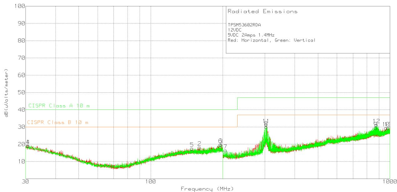
10-6. Radiated Emissions 12-V Input, 5-V Output, 2-A Load
