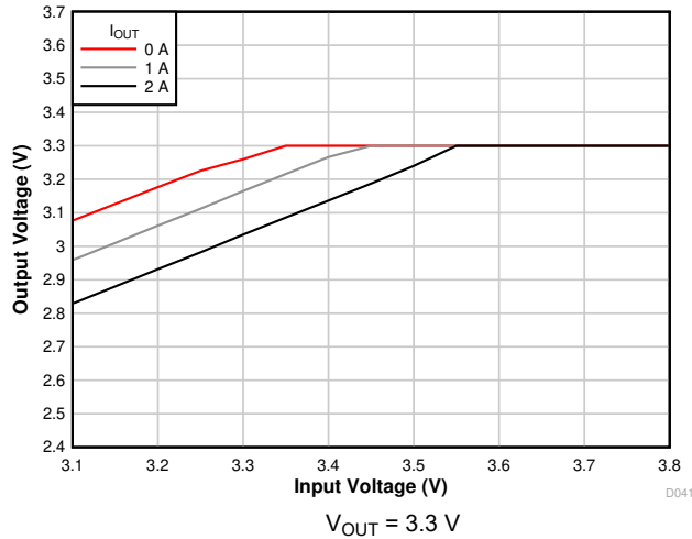
7-7. Voltage Dropout
