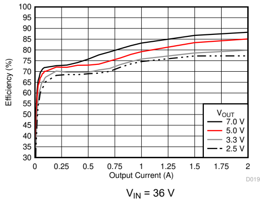
6-17. Efficiency versus Output Current
