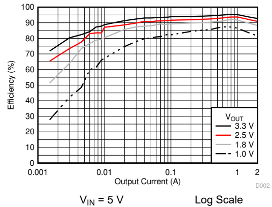
6-2. Efficiency versus Output Current
