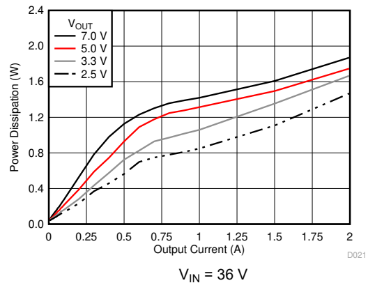
6-19. Power Dissipation versus Output Current
