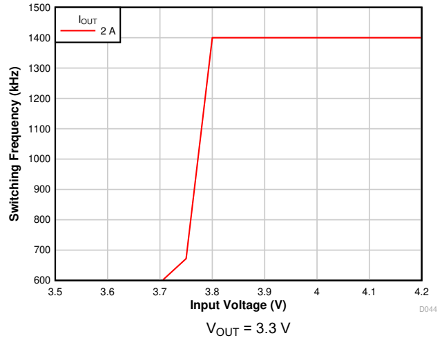
7-8. Frequency Foldback
