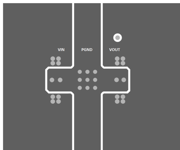
Figure 10-2. Typical Layer-2 Layout
