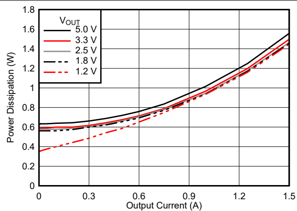
7-18. Power Dissipation
