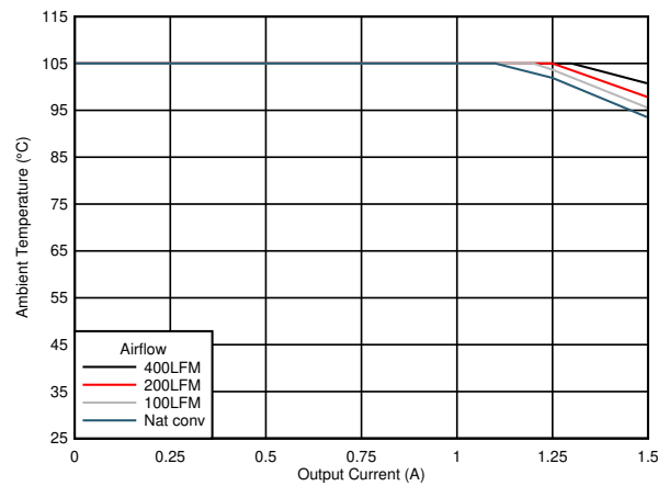
7-10. Safe Operating Area ( V_{OUT} = 1.8\text{ V} )
