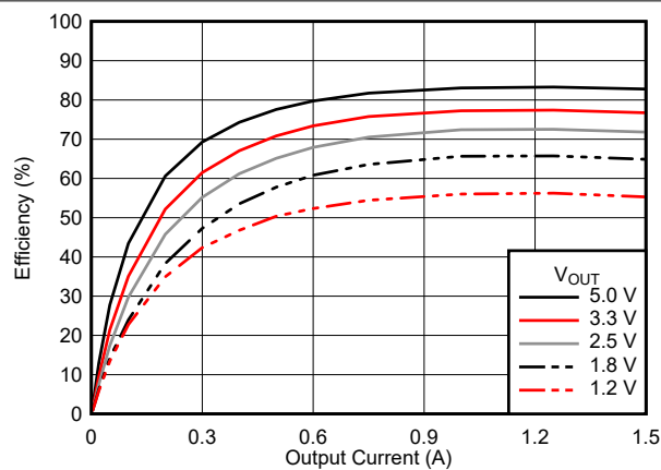
7-17. Efficiency
