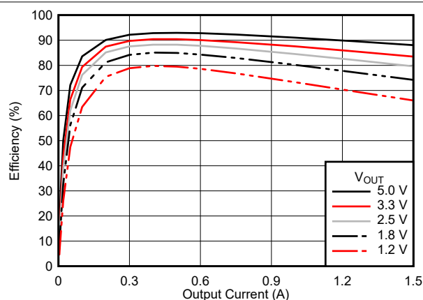
7-1. Efficiency
