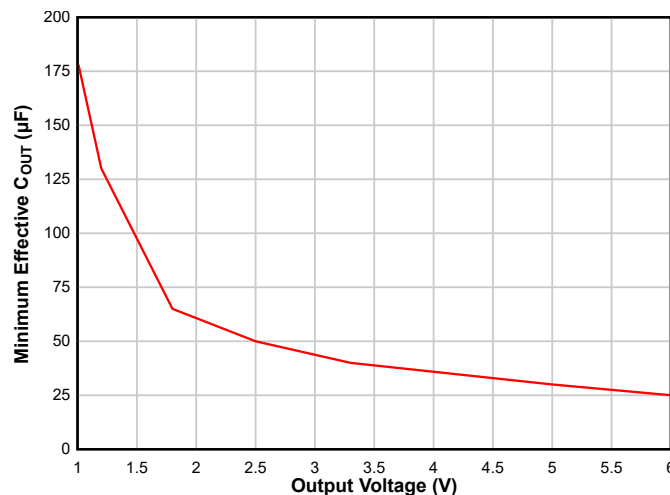
図 8-2. Minimum Required Output Capacitance
