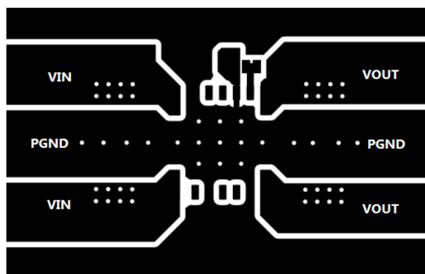
Figure 11-2. Typical Top-Layer
