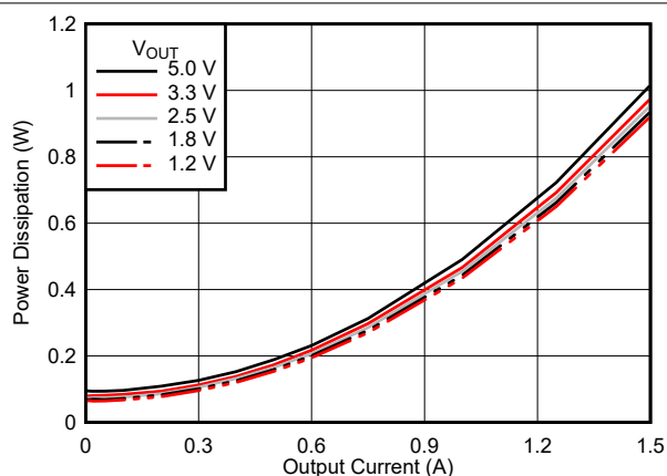
7-2. Power Dissipation
