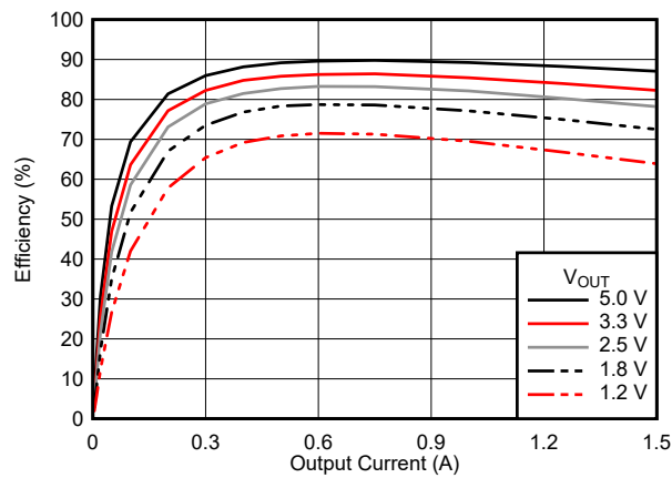
7-7. Efficiency
