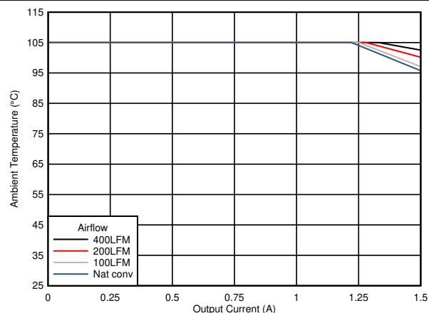
7-4. Safe Operating Area ( V_{OUT} = 1.2\text{ V} )
