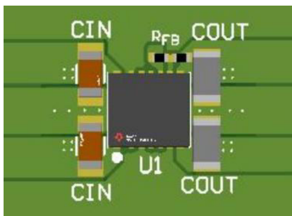
Figure 11-1. Typical Layout
