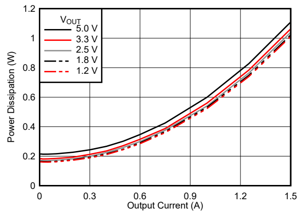
7-8. Power Dissipation
