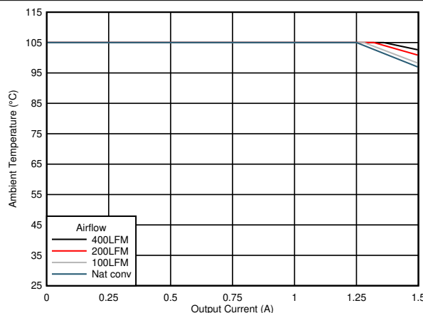
7-5. Safe Operating Area ( V_{OUT} = 3.3\text{ V} )
