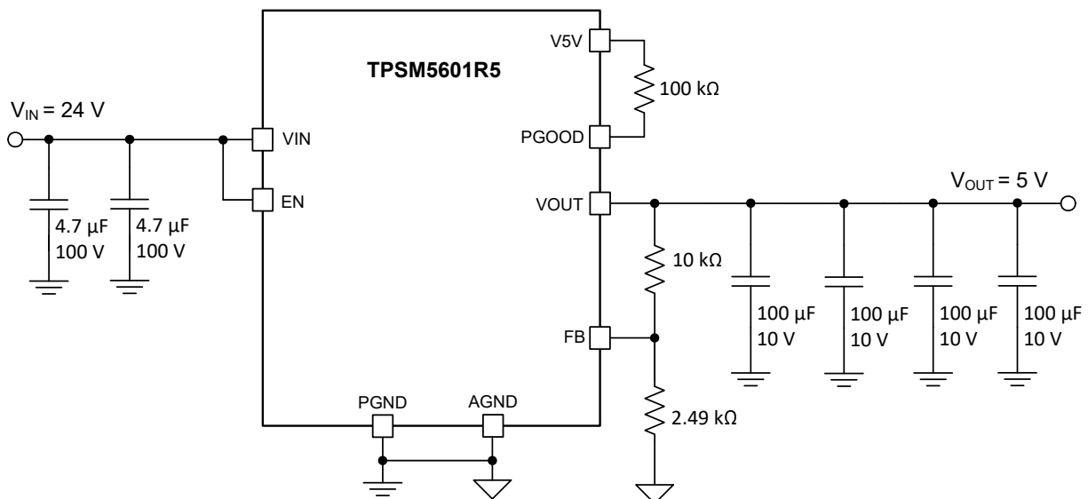
図 9-1. TPSM5601R5 Typical Schematic
