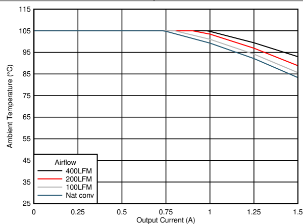
7-15. Safe Operating Area ( V_{OUT} = 3.3\text{ V} )
