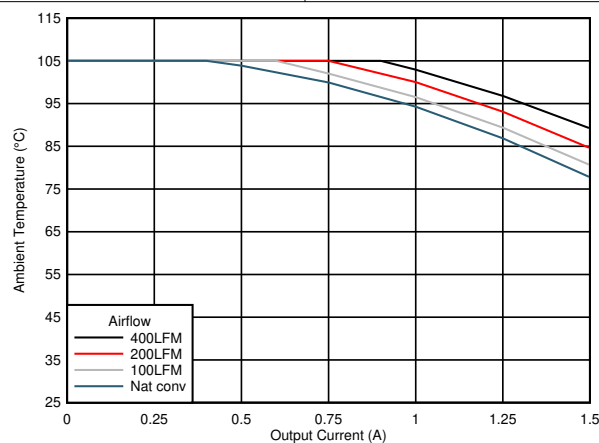
7-20. Safe Operating Area ( V_{OUT} = 3.3\text{ V} )
