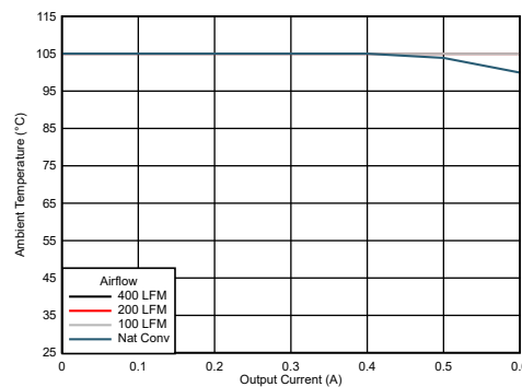
6-17. Safe Operating Area ( V_{OUT} = 5.0\text{ V} )
