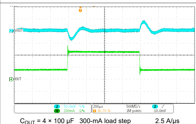
图 8-5. Transient Response Waveform
