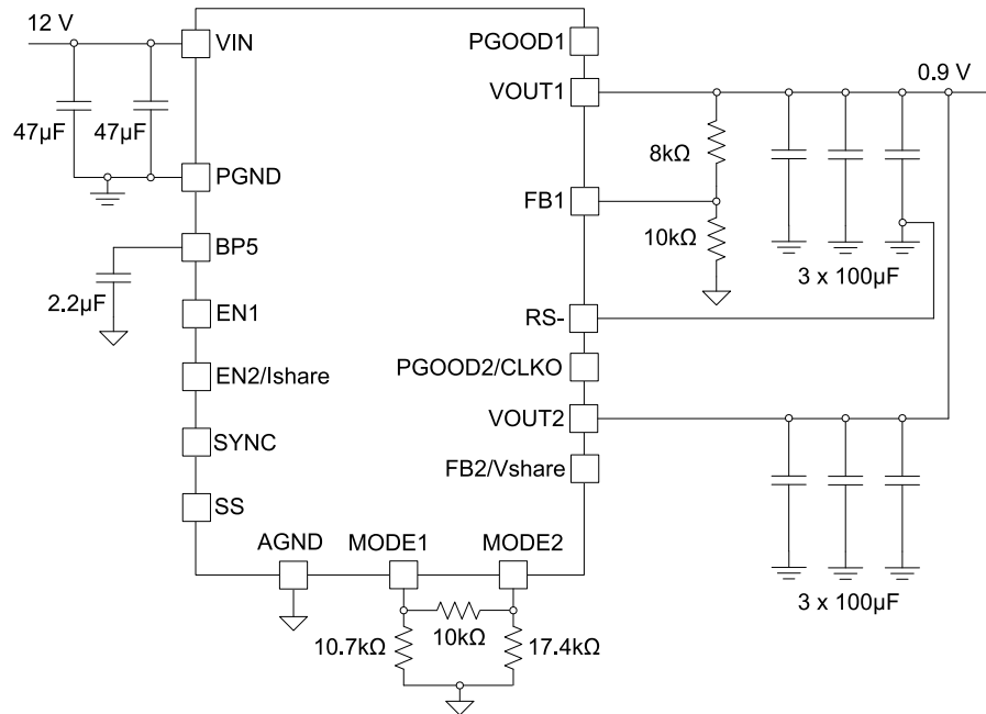
図 8-2. TPSM5D1806 Parallel Outputs Typical Schematic
