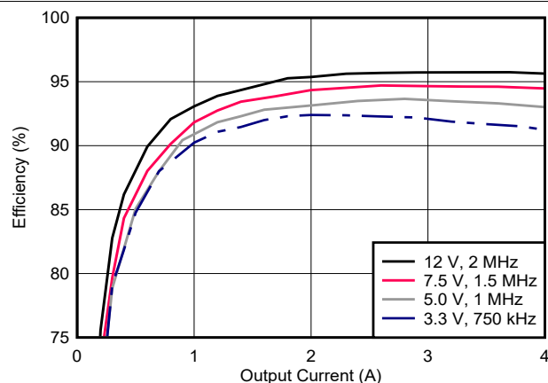
7-14. Efficiency
