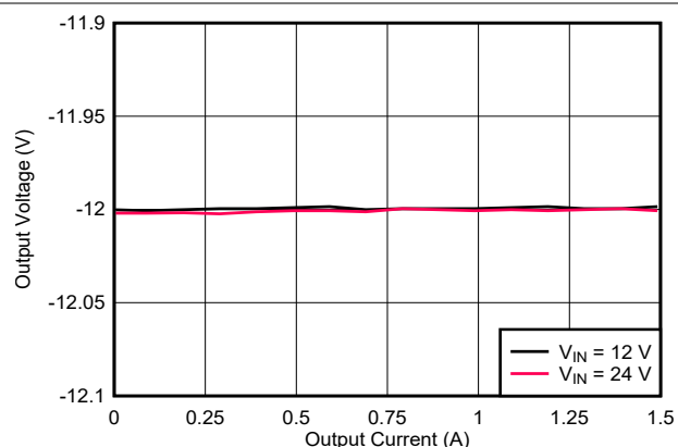
Figure 9-13. Load Regulation
