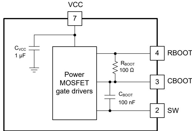
8-4. Internal BOOT Resistor
