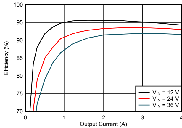
9-2. Efficiency
