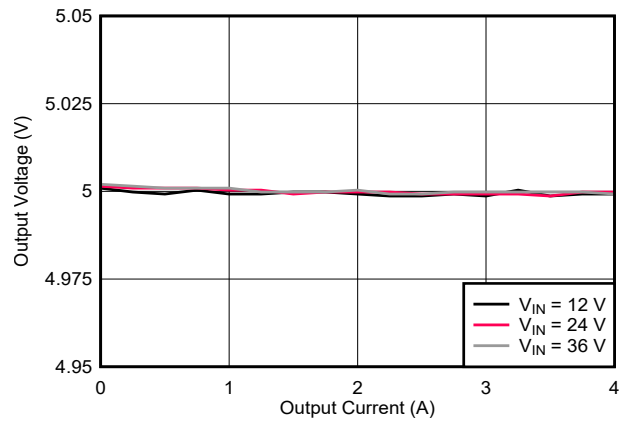
9-3. Load Regulation
