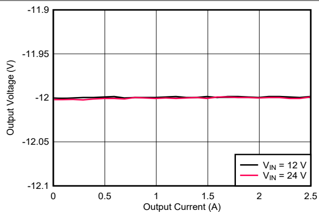
FIG 9-15. Load Regulation
