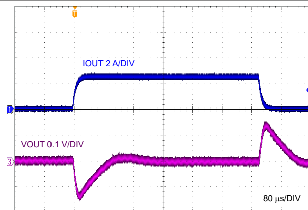
FIG 9-16. Load Transient, 0 A to 2.5 A
