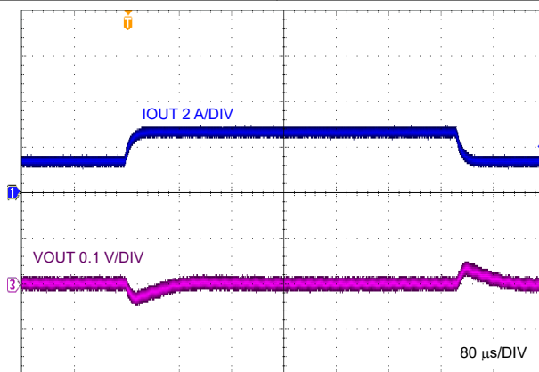
FIG 9-17. Load Transient, 1.25 A to 2.5 A
