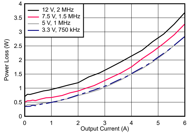
図 7-15. Power Dissipation
