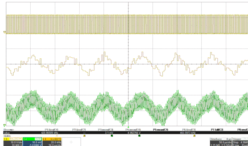
図 8-3. Output Ripple Without Ripple Cancellation Showing V_{\text{sw}} (Top), F_{\text{sw}} (Middle), V_{\text{out}} (Bottom)
