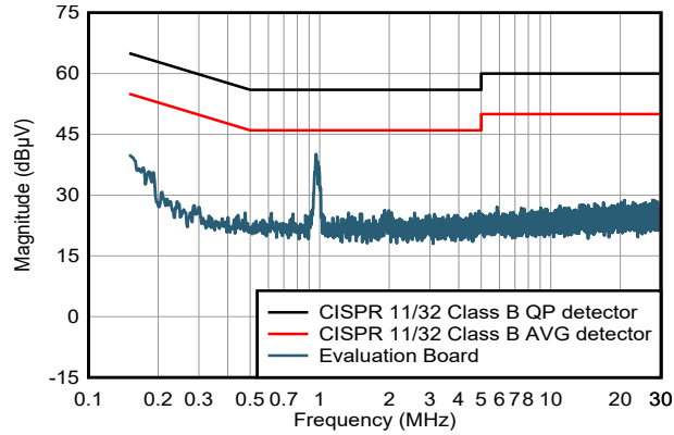
図 9-8. CISPR 11/32 Class B Conducted Emissions: V_{IN} = 24\text{ V} , SPSP ON TPSM63610EVM
