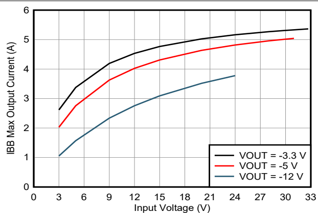
図 9-13. IBB Maximum Output Current
