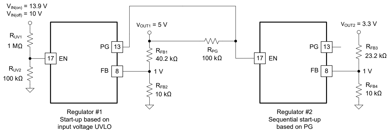
図 8-5. TPSM63608 Sequencing Implementation Using PG and EN
