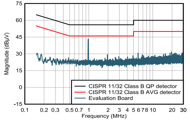
図 9-9. CISPR 11/32 Class B Conducted Emissions: V_{IN} = 24\text{ V} , SPSP OFF TPSM63610EVM
