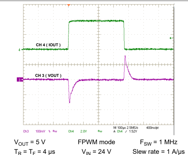
Figure 9-7. Load Transient, 0\text{ A} to 4\text{ A} , 1\text{ A}/\mu\text{s}
