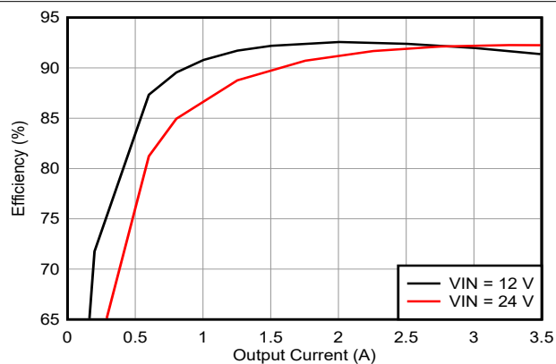
図 9-14. Efficiency for V_{OUT} = -12\text{ V} , FPWM Mode
