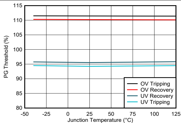
図 7-7. Power-Good (PG) Thresholds
