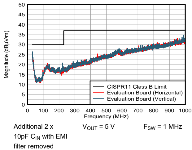
図 9-10. CISPR 11 Class B Radiated Emissions: V_{IN} = 24\text{ V} , SPSP ON TPSM63610EVM
