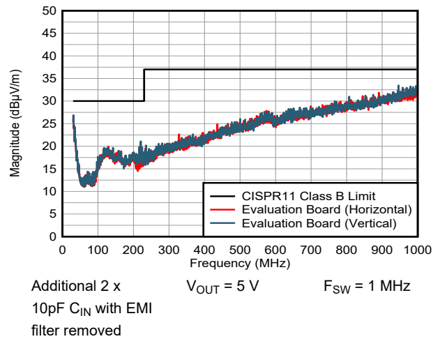
図 9-11. CISPR 11 Class B Radiated Emissions: V_{IN} = 24\text{ V} , SPSP OFF TPSM63610EVM
