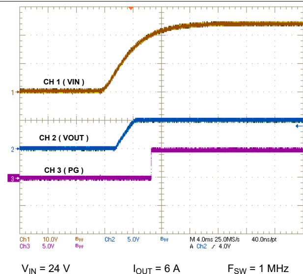
Figure 9-6. Start-up
