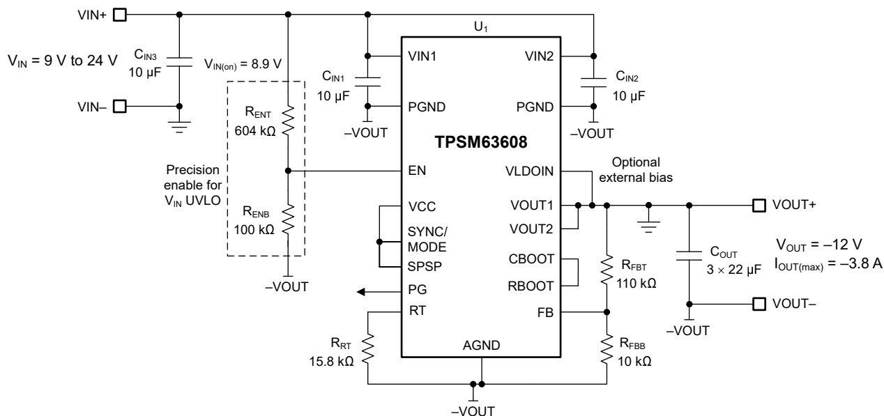
図 9-12. Circuit Schematic
