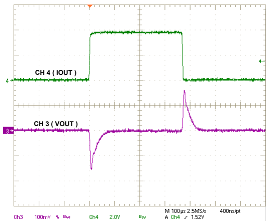
8-8. Load Transient, 0 A to 4 A, 1 A/ \mu s
