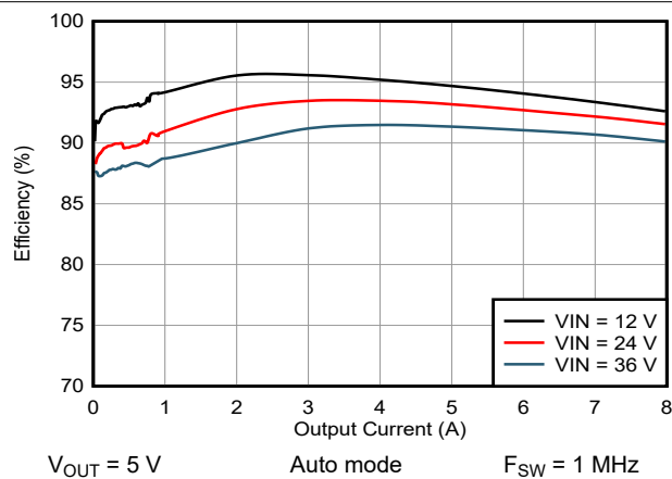
図 9-3. Efficiency for V_{OUT} = 5\text{ V}
