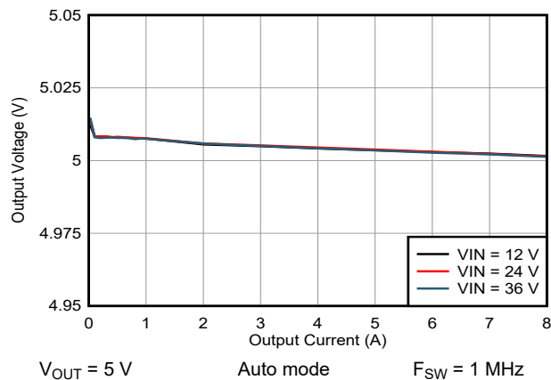
図 9-5. Load Regulation for V_{OUT} = 5\text{ V}
