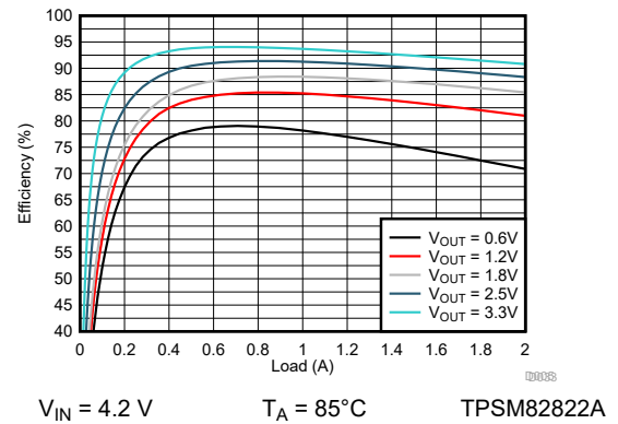
FIG 9-89. Efficiency
