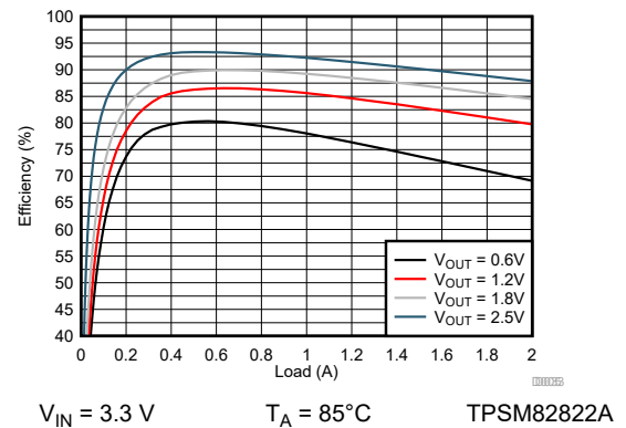
FIG 9-91. Efficiency
