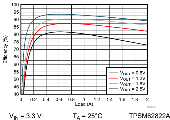
FIG 9-90. Efficiency
