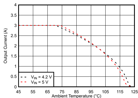
图 9-146. Safe Operating Area
