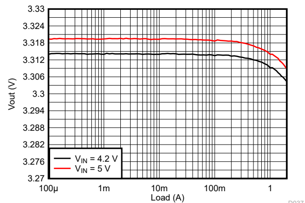
9-101. Load Regulation
