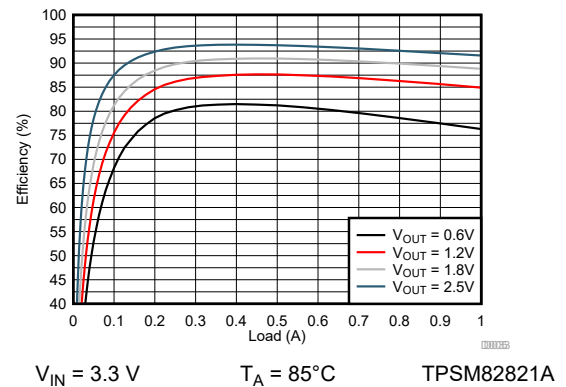
Figure 9-34. Efficiency
