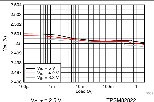
9-69. Load Regulation
