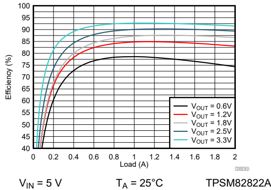
FIG 9-86. Efficiency
