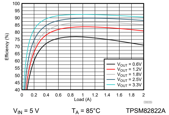
FIG 9-87. Efficiency
