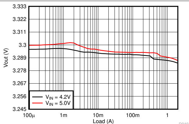
9-68. Load Regulation
