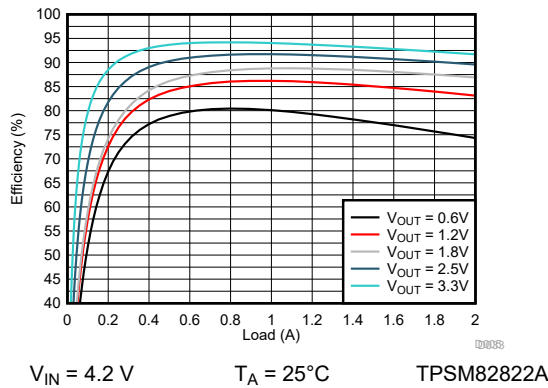
FIG 9-88. Efficiency
