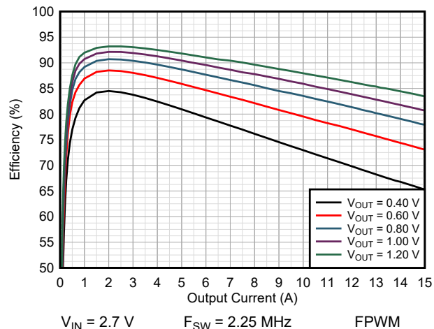
9-15. Efficiency TPSM8287A15BBH
