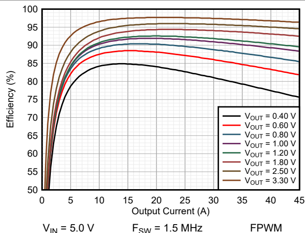
9-55. Efficiency
