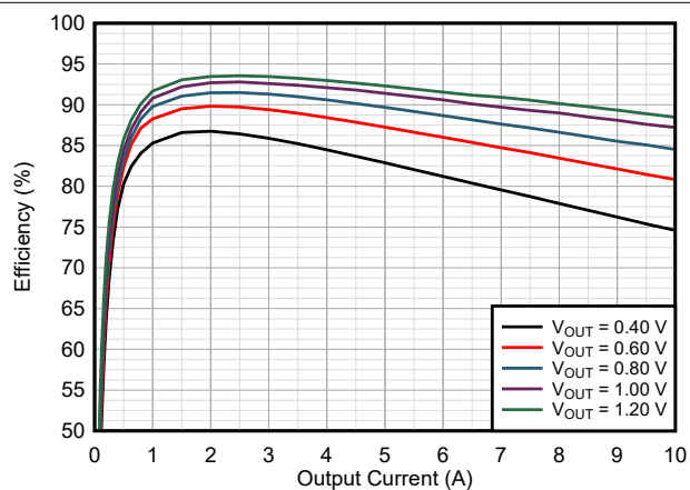
図 9-3. Efficiency TPSM8287A10BAH
