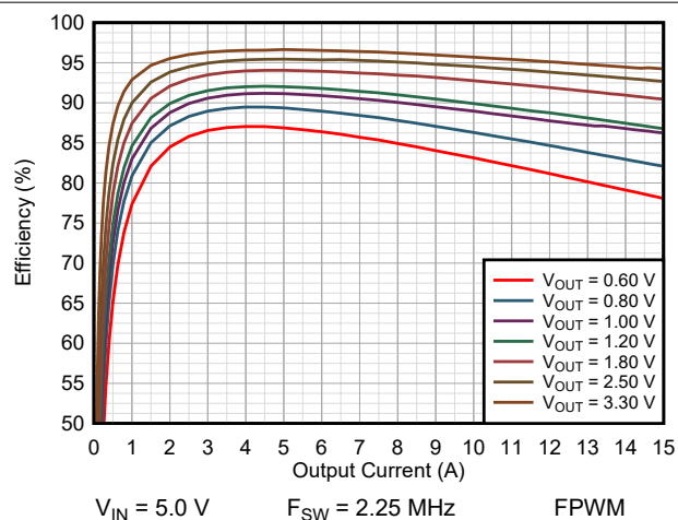
9-19. Efficiency TPSM8287A15BBH
