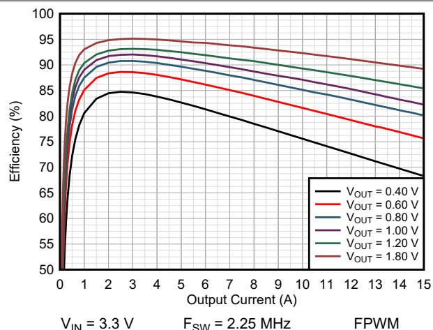
9-17. Efficiency TPSM8287A15BBH
