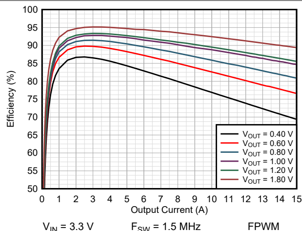
9-16. Efficiency TPSM8287A15BAH
