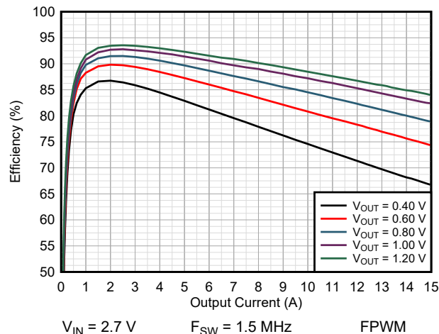
9-14. Efficiency TPSM8287A15BAH
