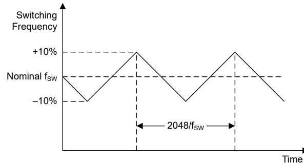
図 7-16. Spread Spectrum Clocking Behavior
