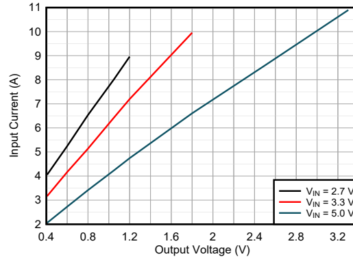
FIG 7-18. TPSM8287A12BBS Typical Input Current in Current Limit
