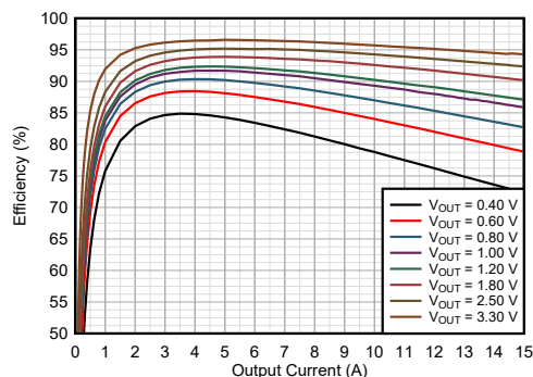
効率性 TPSM8287A15BAH (V IN = 5.0V、FPWM)
