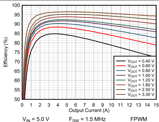
9-18. Efficiency TPSM8287A15BAH
