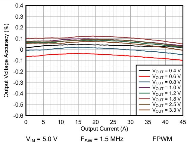
9-56. Load Regulation
