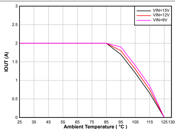
Auto PFM/PWM F_{sw} = 2.5\text{ MHz} 8-45. Thermal Derating V_{OUT} = 1.2\text{ V}
