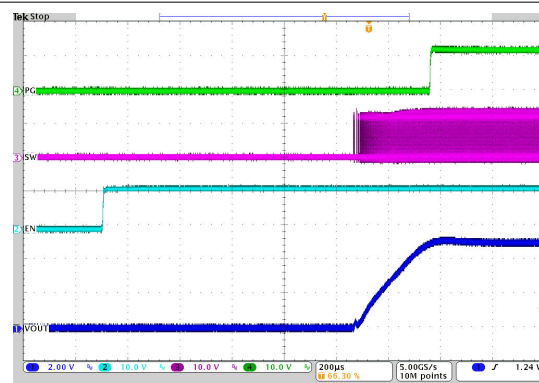
8-26. Start-Up Timing
