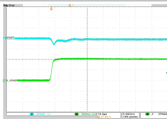
8-38. PSM-to-PWM Transition
