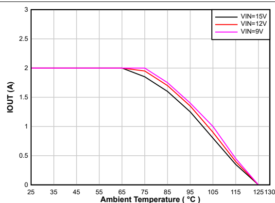
Auto PFM/PWM F_{sw} = 2.5\text{ MHz} 8-46. Thermal Derating V_{OUT} = 3.3\text{ V}
