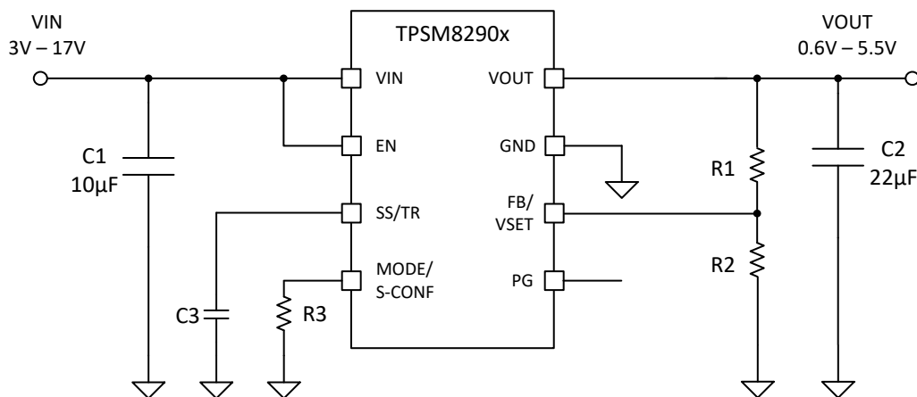
図 8-1. Typical Application Circuit
