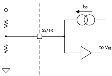
図 8-3. Tracking Operation Simplified Schematic
