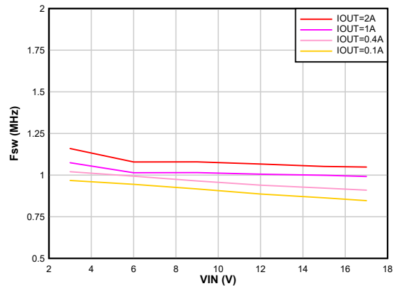
8-17. Switching Frequency vs Input Voltage V_{OUT} = 1.2 V
