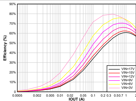
8-55. Efficiency vs Output Current V_{OUT} = 0.4 \text{ V}
