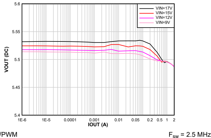
8-60. Output Voltage vs Output Current V_{OUT} = 5.5\text{ V}
