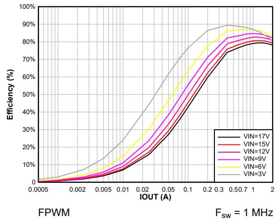
8-7. Efficiency vs Output Current V_{OUT} = 1.2 \text{ V}
