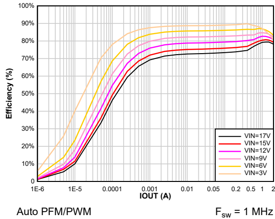
8-5. Efficiency vs Output Current V_{OUT} = 1.2 \text{ V}
