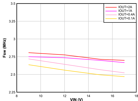
8-24. Switching Frequency vs Input Voltage V_{OUT} = 5.5 \text{ V}
