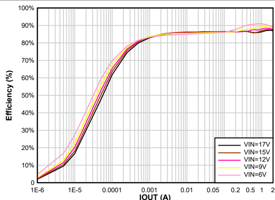
8-11. Efficiency vs Output Current V_{OUT} = 3.3 \text{ V}
