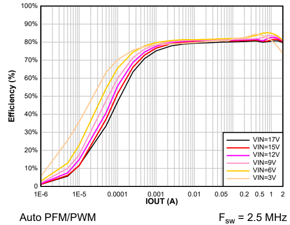
8-6. Efficiency vs Output Current V_{OUT} = 1.2 \text{ V}
