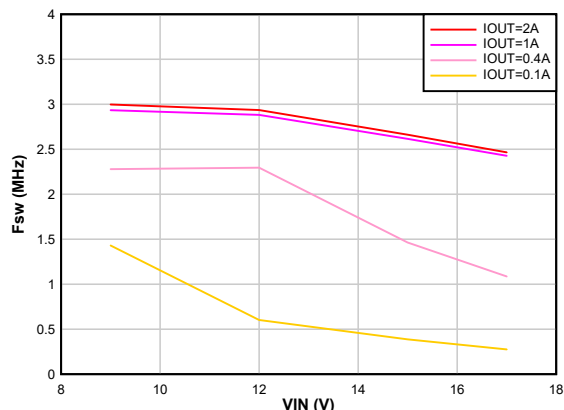
8-23. Switching Frequency vs Input Voltage V_{OUT} = 5.5 \text{ V}
