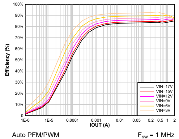
8-8. Efficiency vs Output Current V_{OUT} = 1.8 \text{ V}
