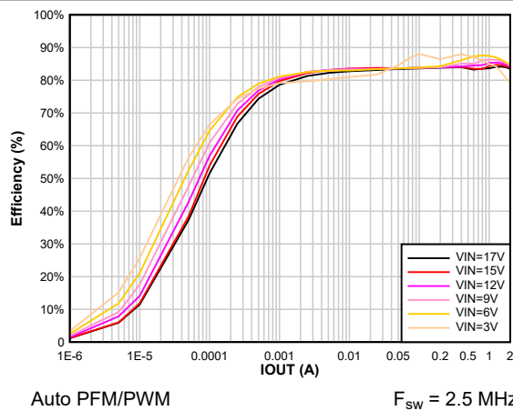
8-9. Efficiency vs Output Current V_{OUT} = 1.8 \text{ V}
