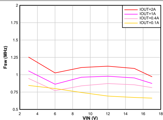
8-56. Switching Frequency vs Input Voltage V_{OUT} = 0.4 \text{ V}
