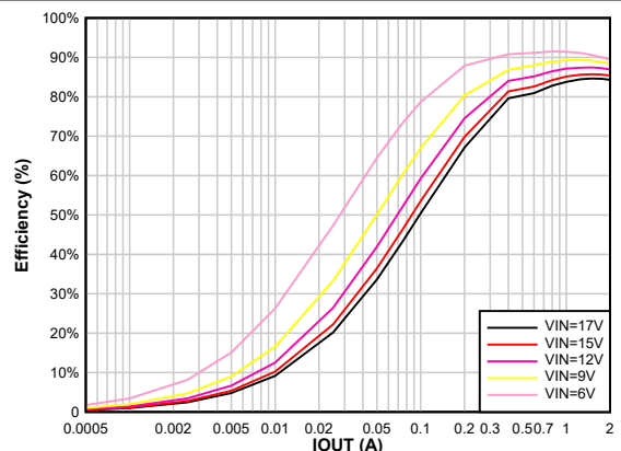
8-12. Efficiency vs Output Current V_{OUT} = 3.3 \text{ V}
