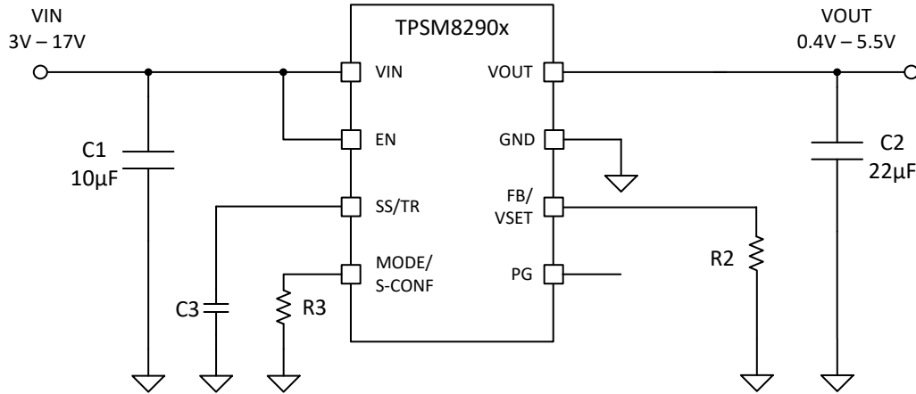
図 7-3. Setable V_O Operation Schematic
