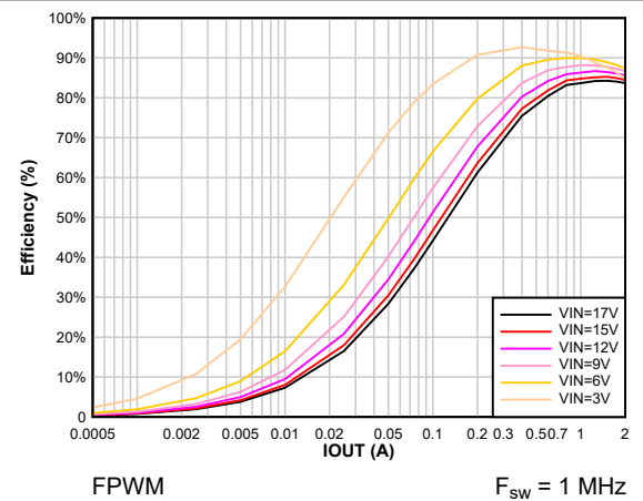
8-10. Efficiency vs Output Current V_{OUT} = 1.8 \text{ V}
