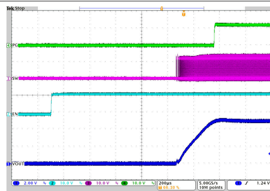
8-26. Start-Up Timing
