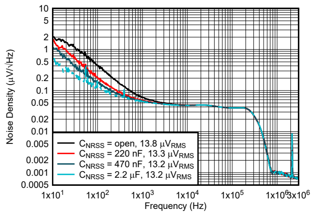
Figure 6-28. Output Noise Density vs Frequency
