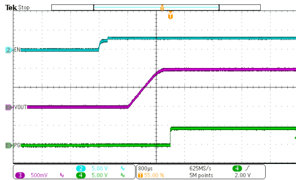
7-11. EN Start-Up – With Load
