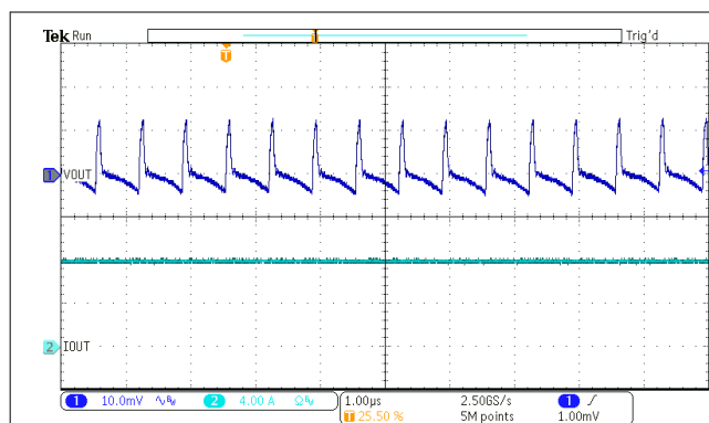
7-16. Output Ripple – 8-A Load
