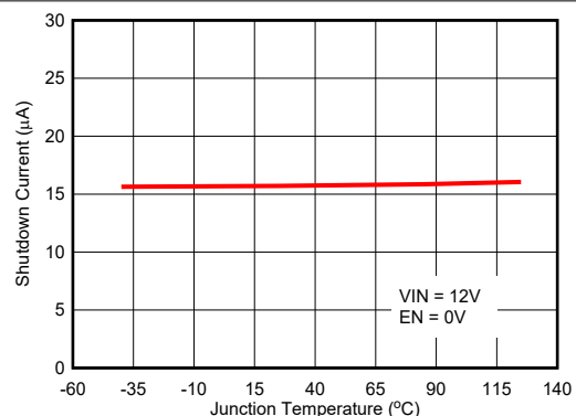
図 5-13. Shutdown Current
