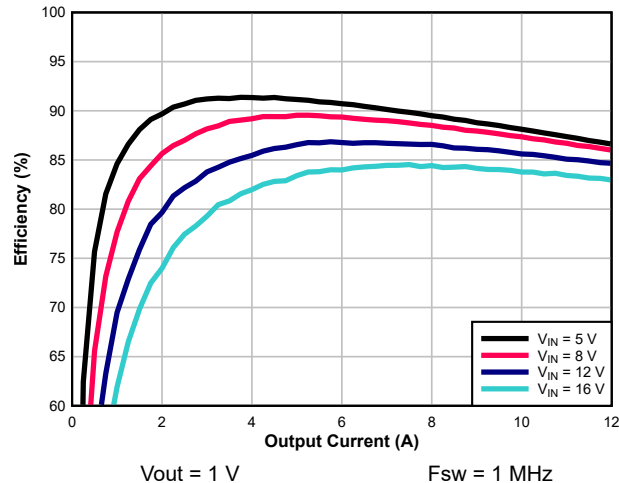
图 8-4. Efficiency Curves
