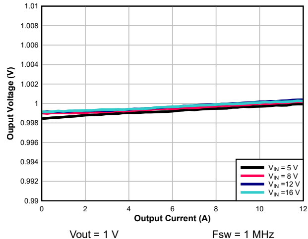
图 8-5. Load Regulation
