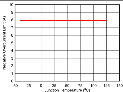
图 6-4. Negative Overcurrent Limit
