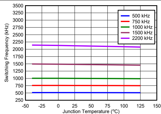
图 6-16. Switching Frequency vs Temperature
