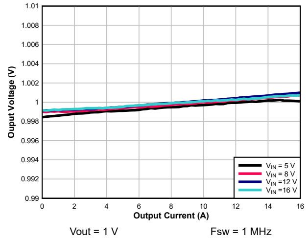
8-5. Load Regulation
