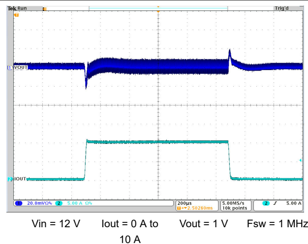
8-8. Load Transient
