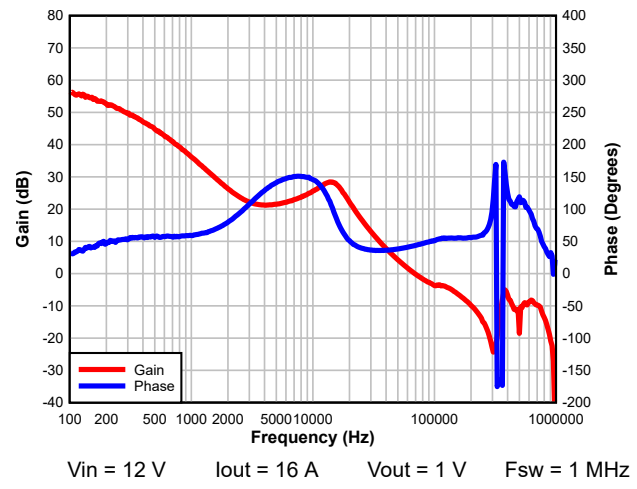
8-7. Bode Plot
