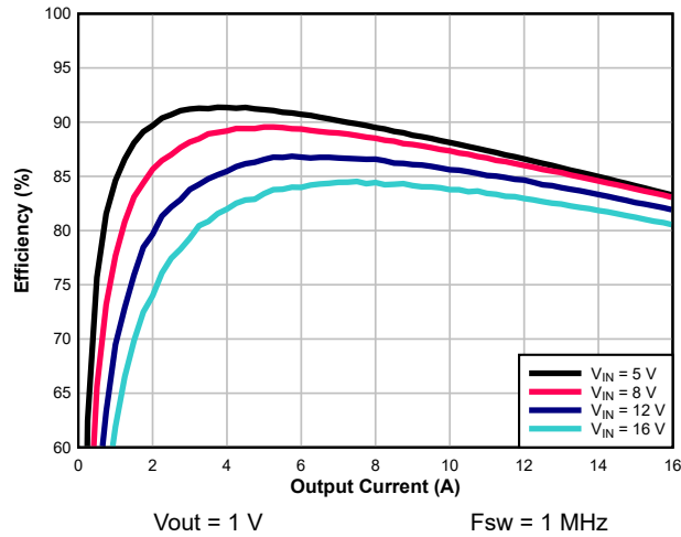
8-4. Efficiency Curves
