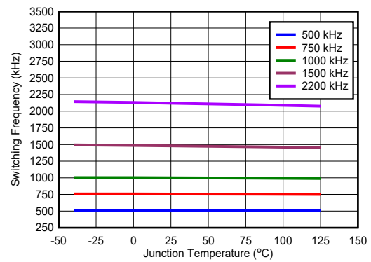
6-16. Switching Frequency vs Temperature
