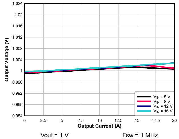
图 8-5. Load Regulation
