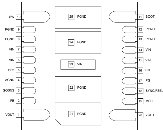
✎ 5-1. 25-Pin B3QFN-RDG Package (Bottom View)
