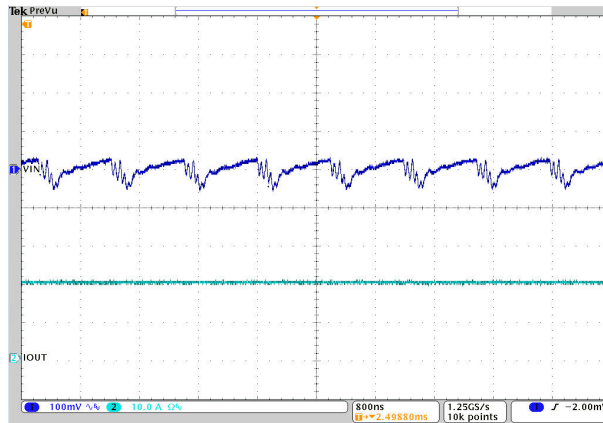
8-16. Input Ripple – Full Load
