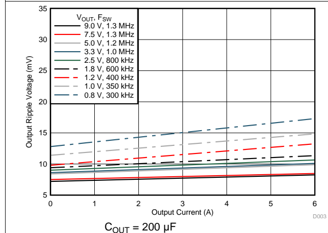
FIG 3. Ripple Voltage vs Output Current
