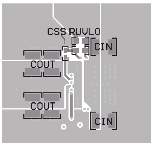
Figure 30. Typical Bottom-Layer Layout (Bottom View)
