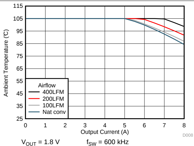
FIG 4. Safe Operating Area
