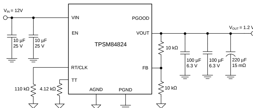
図 24. TPSM84824 Typical Application
