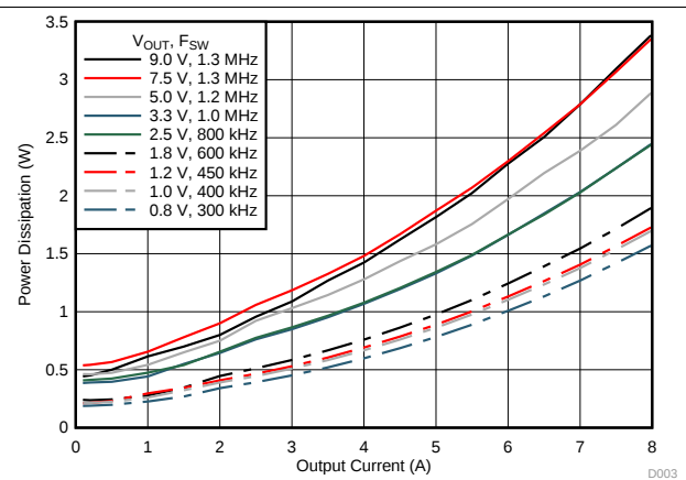
FIG 2. Power Dissipation vs Output Current
