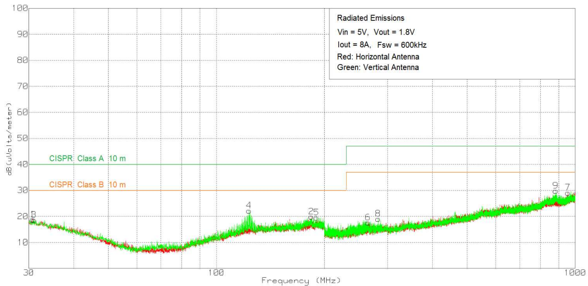
✎ 33. Radiated Emissions 5-V Input, 1.8-V Output, 8-A Load (EN55011 Class B)
