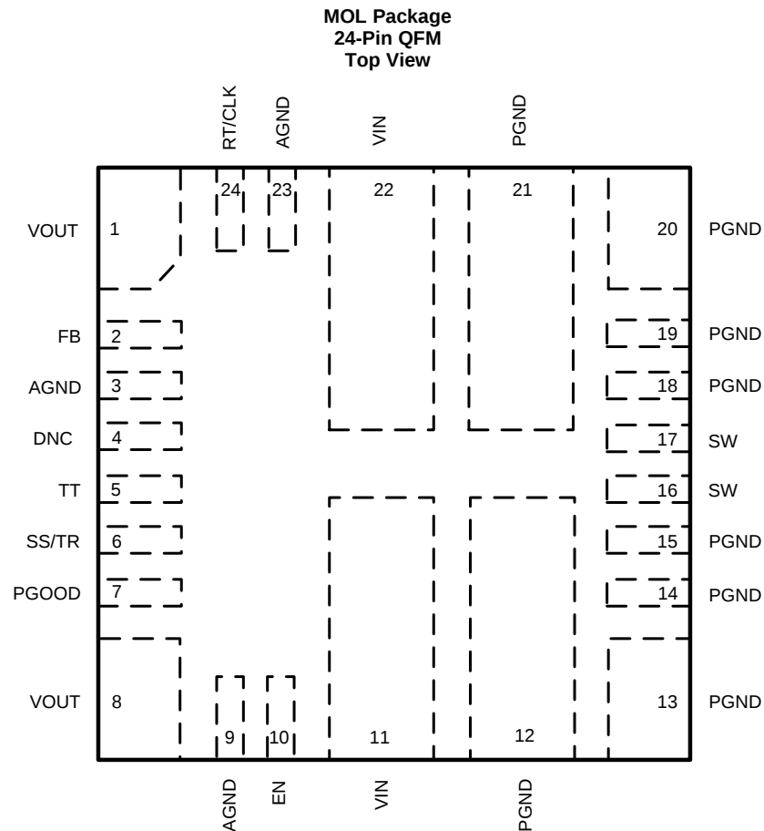
Pin Functions
