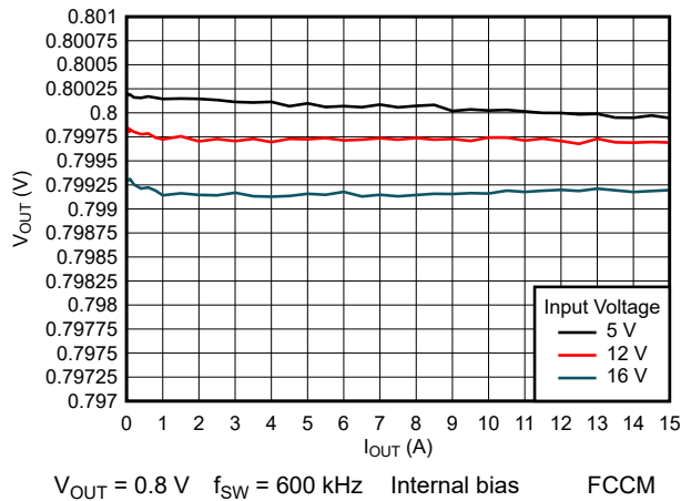
8-12. Load Regulation
