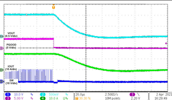
I OUT = 15 A FCCM 8-36. Shutdown Through Enable
