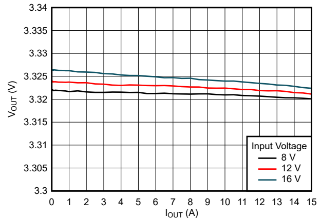
Figure 8-17. Load Regulation
