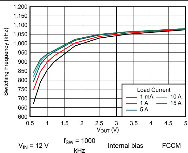
图 8-25. Switching Frequency
