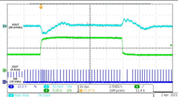
I STEP = 7.5 A - 15 A - 7.5 A 5 A/µs 8-37. Transient Response, V PP = 74 mV
