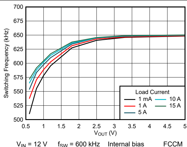
图 8-24. Switching Frequency
