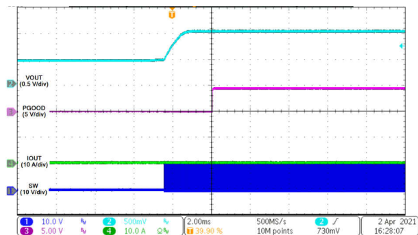
I OUT = 0 A FCCM 8-35. Startup Through Enable into Prebiased Load
