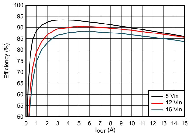
图 8-5. Efficiency
