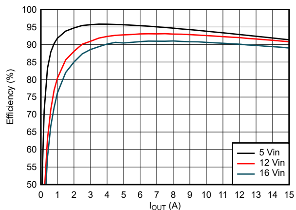
图 8-5. Efficiency
