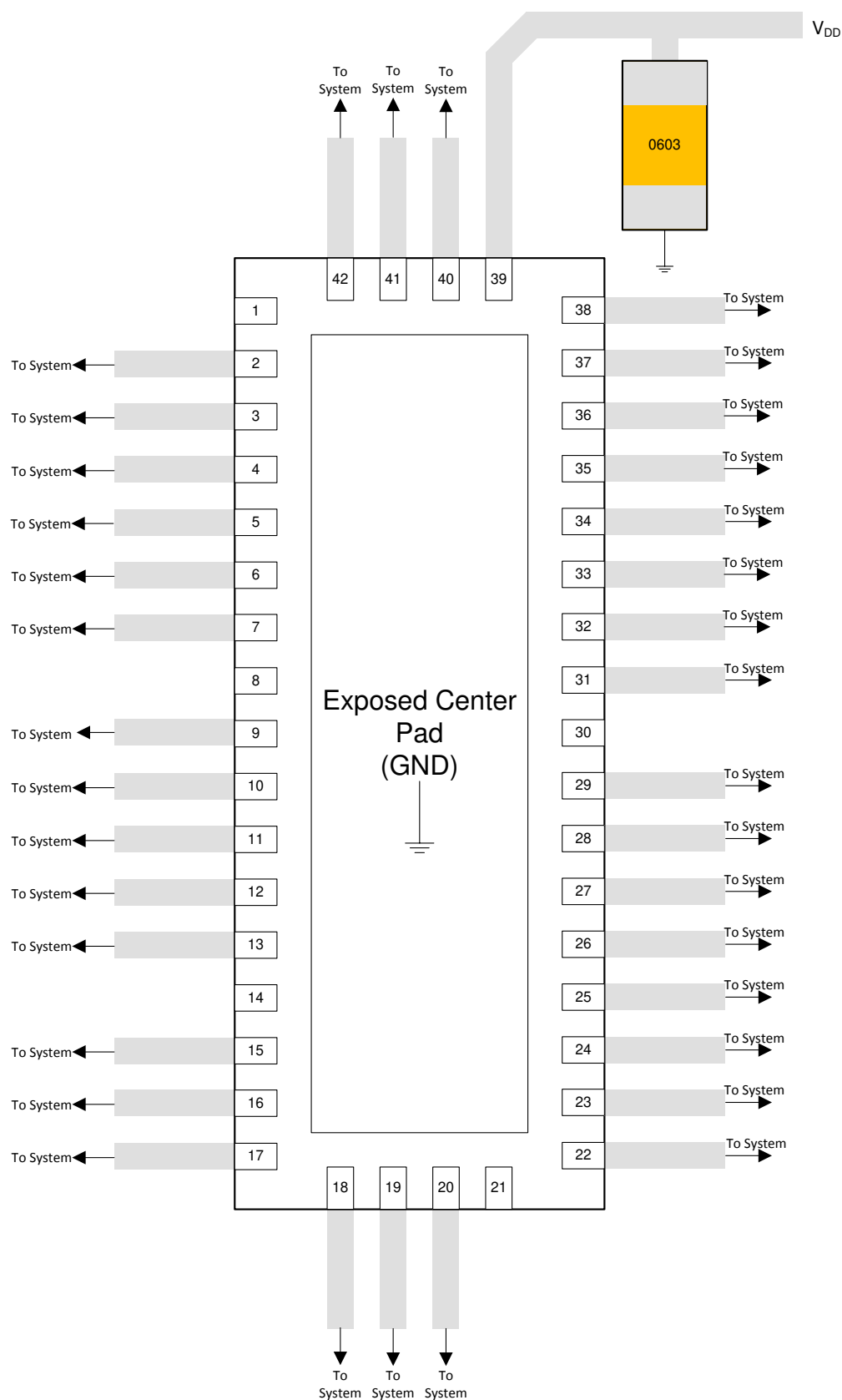
11-2. Layout Example
