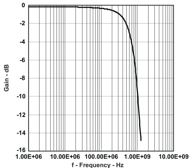
FIG 9-2. Gain vs Frequency
