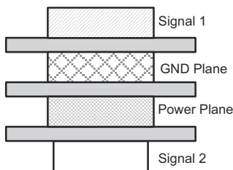
Figure 11-1. Four-Layer Board Stackup
