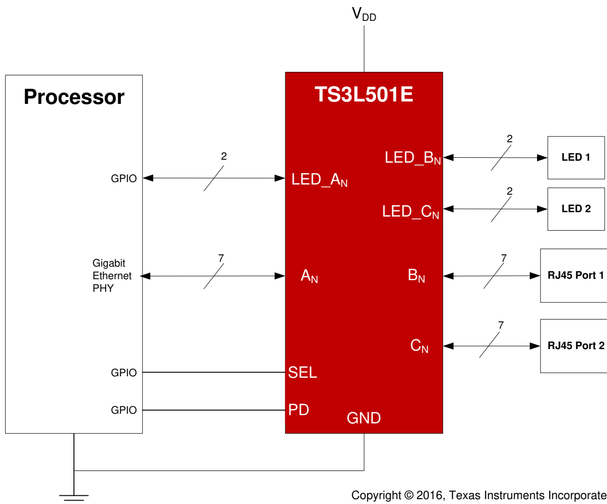
図 9-1. Typical Application Schematic
