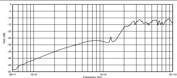
5-3. Crosstalk
