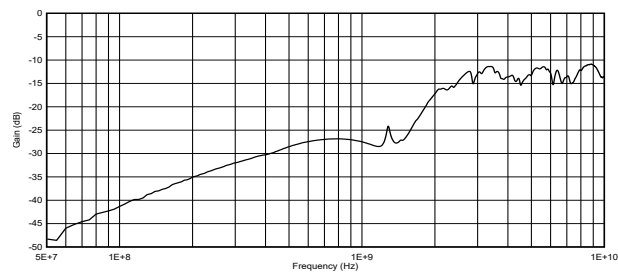
5-2. OFF Isolation
