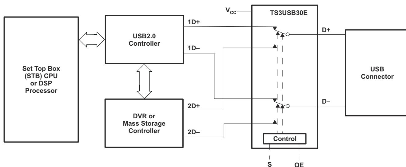
図 8-1. Application Diagram
