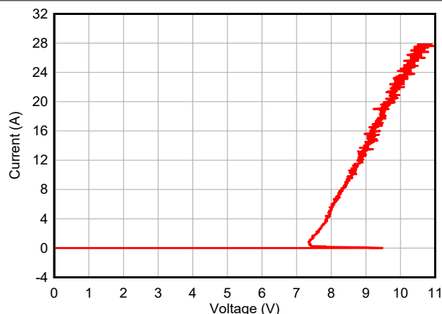
図 5-1. Positive TLP Curve - TSD05C
