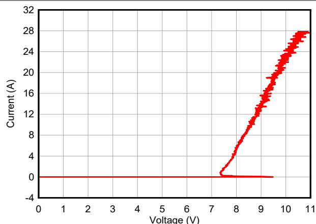
図 5-2. Negative TLP Curve - TSD05C
