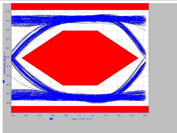
図 5-3. 2 Meter Post-Channel With TUSB211A-Q1 EQ=1
