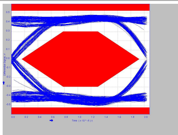
図 5-1. 2 Meter Pre-Channel With TUSB211A-Q1 EQ=1
