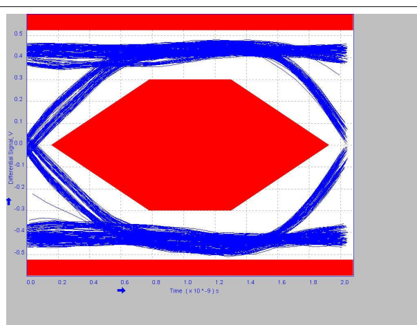
図 7-4. 2 Meter Pre-Channel With TUSB211A-Q1 EQ=1
