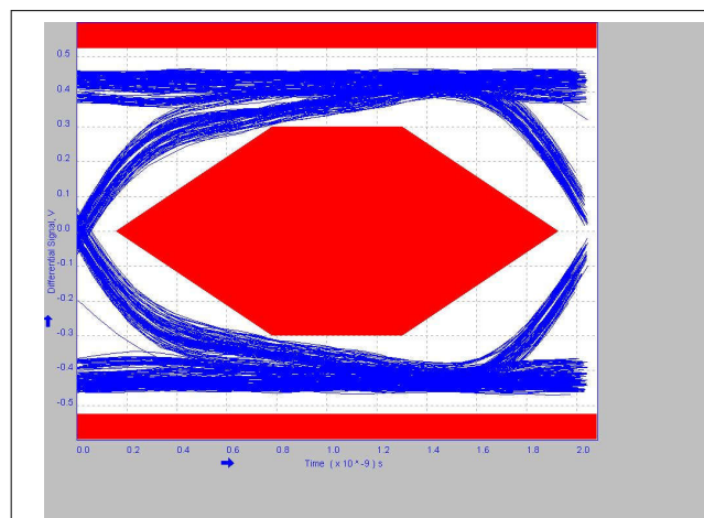
図 7-3. 2 Meter Pre-Channel Without TUSB211A-Q1
