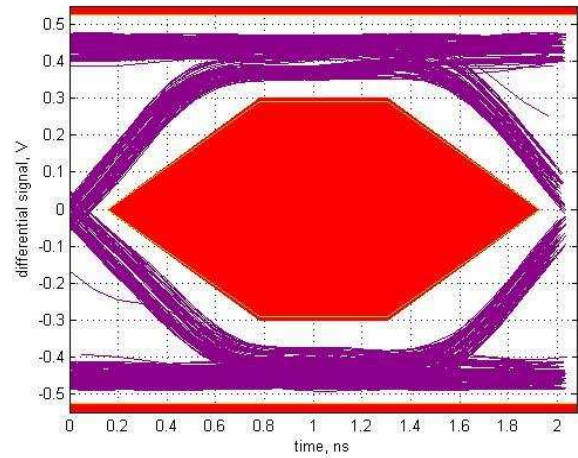
FIG 15. High DC Boost, AC Boost Level 1
