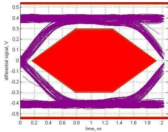
FIG 13. Low DC Boost, AC Boost Level 1
