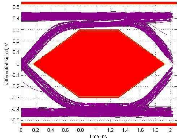
FIG 11. Mid DC Boost, AC Boost Level 0
