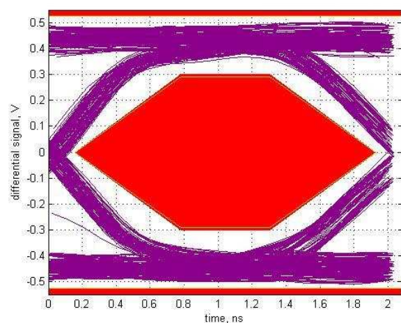
FIG 12. High DC Boost, AC Boost Level 0
