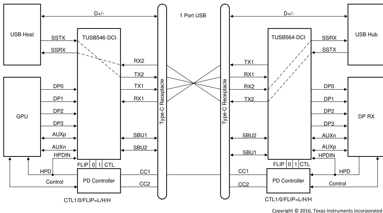
8-5. USB3.1 Only – With Flip (CTL1 = L, CTL0 = H, FLIP = H)
