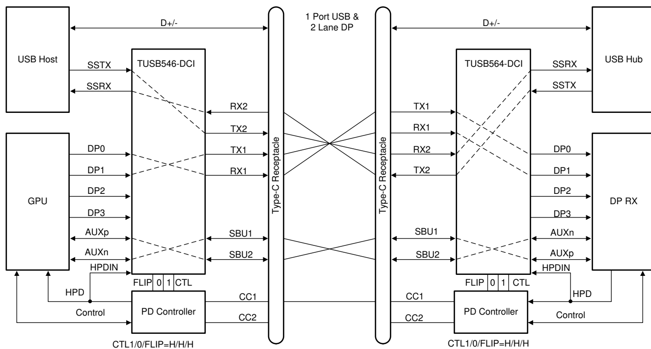
8-7. USB 3.1 + 2 Lane DP – Flip (CTL1 = H, CTL0 = H, FLIP = H)
