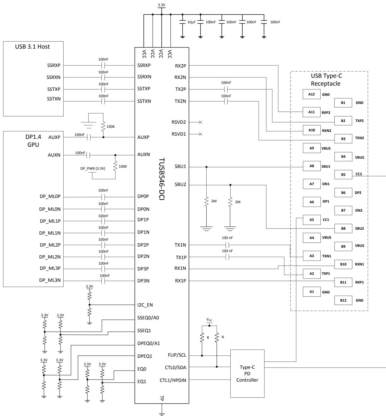
8-2. Application Circuit
