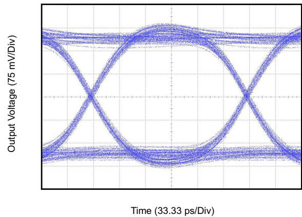
6-10. USB 3.1 Gen1 Eye-Pattern Performance with 12-inch Input PCB Trace at 5 Gbps
