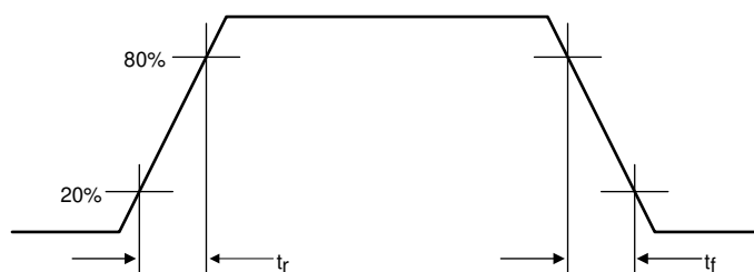
FIG 7-5. Output Rise and Fall Times
