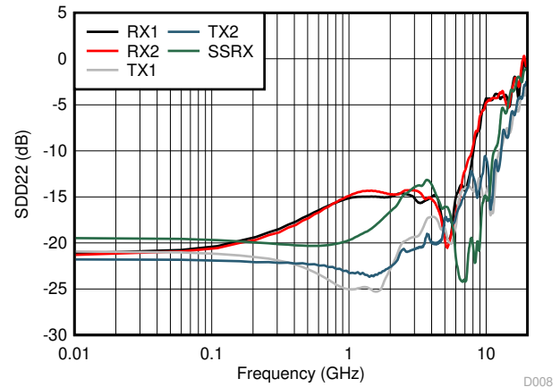
6-8. Output Return Loss Performance
