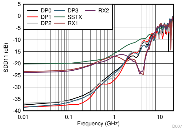
6-7. Input Return Loss Performance
