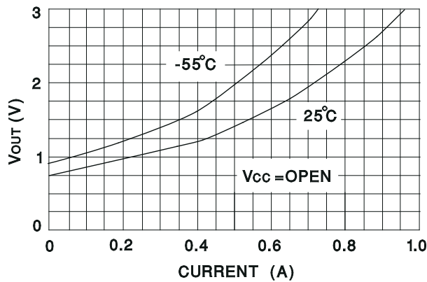
7-3. Output Voltage vs Output Current
