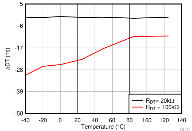
5-25. Dead Time Matching vs Temperature (with R_{DT} = 20\text{ k}\Omega and 100\text{ k}\Omega )
