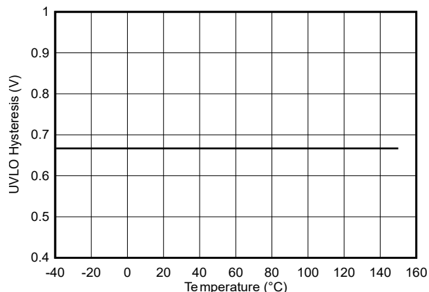
図 5-19. VDD 8-V UVLO Hysteresis vs Temperature
