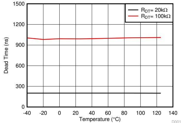
5-24. Dead Time vs Temperature (with R_{DT} = 20\text{ k}\Omega and 100\text{ k}\Omega )
